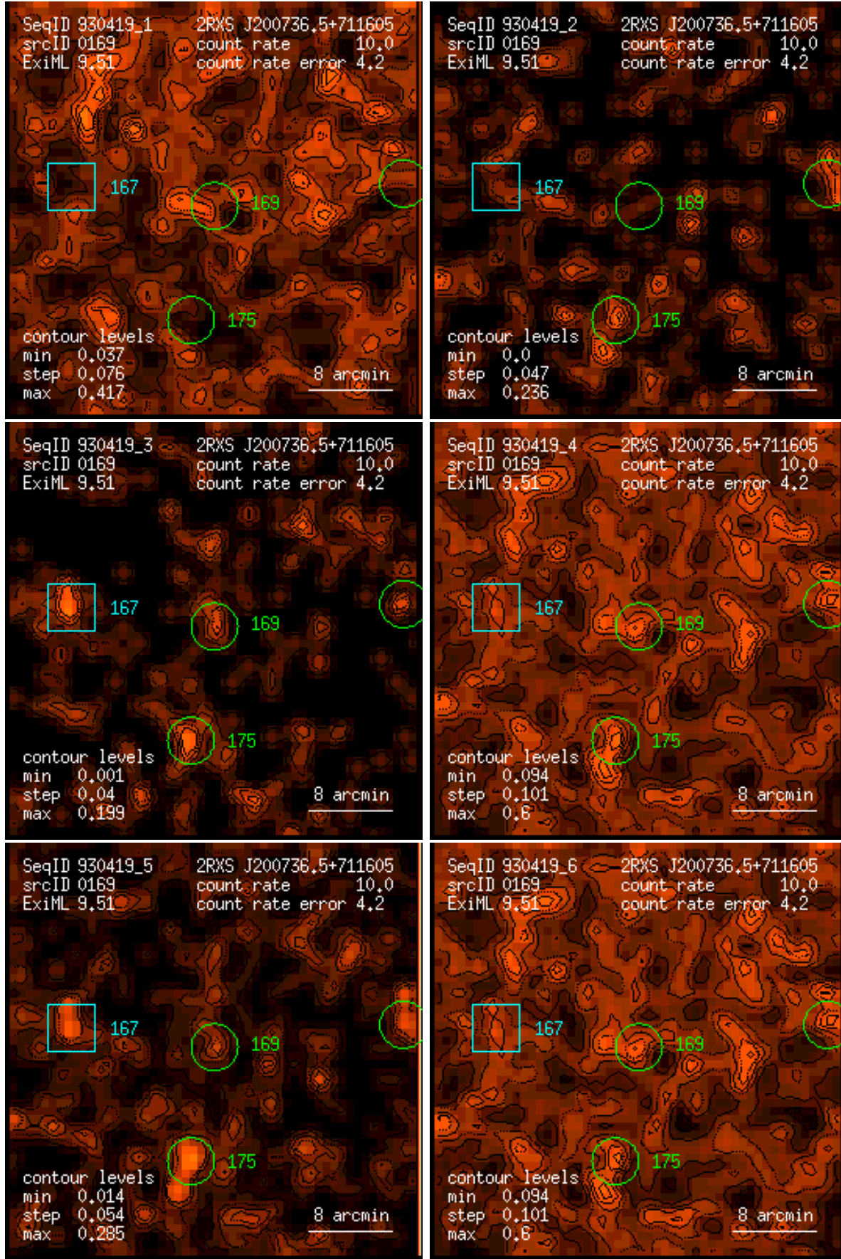
Figure 169: RASS 930419: detection 0169: band rate images, Gaussian filter: (1) PSPC channels 11 – 41, (2) 52 – 90, (3) 91 – 201, (4) 11 – 235, (5) 52 – 201, (6) 11 – 201. Broad band rates in counts/ks. Band rate contour levels in counts/ks/arcmin 2 .
