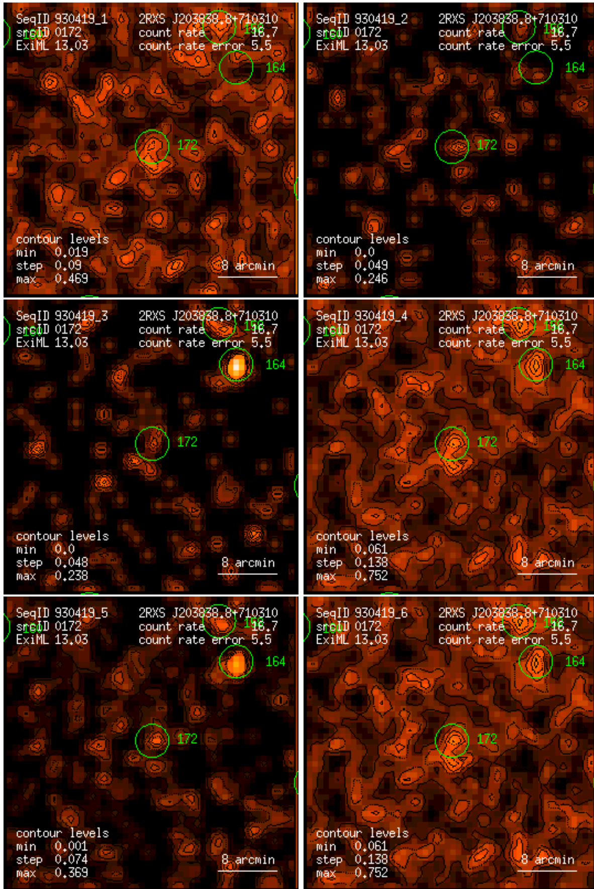
Figure 172: RASS 930419: detection 0172: band rate images, Gaussian filter: (1) PSPC channels 11 – 41, (2) 52 – 90, (3) 91 – 201, (4) 11 – 235, (5) 52 – 201, (6) 11 – 201. Broad band rates in counts/ks. Band rate contour levels in counts/ks/arcmin 2 .
