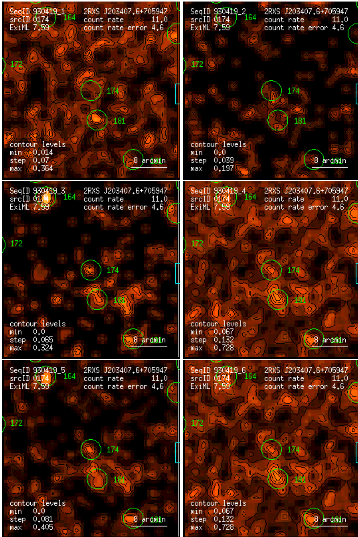
Figure 174: RASS 930419: detection 0174: band rate images, Gaussian filter: (1) PSPC channels 11 – 41, (2) 52 – 90, (3) 91 – 201, (4) 11 – 235, (5) 52 – 201, (6) 11 – 201. Broad band rates in counts/ks. Band rate contour levels in counts/ks/arcmin 2 .
