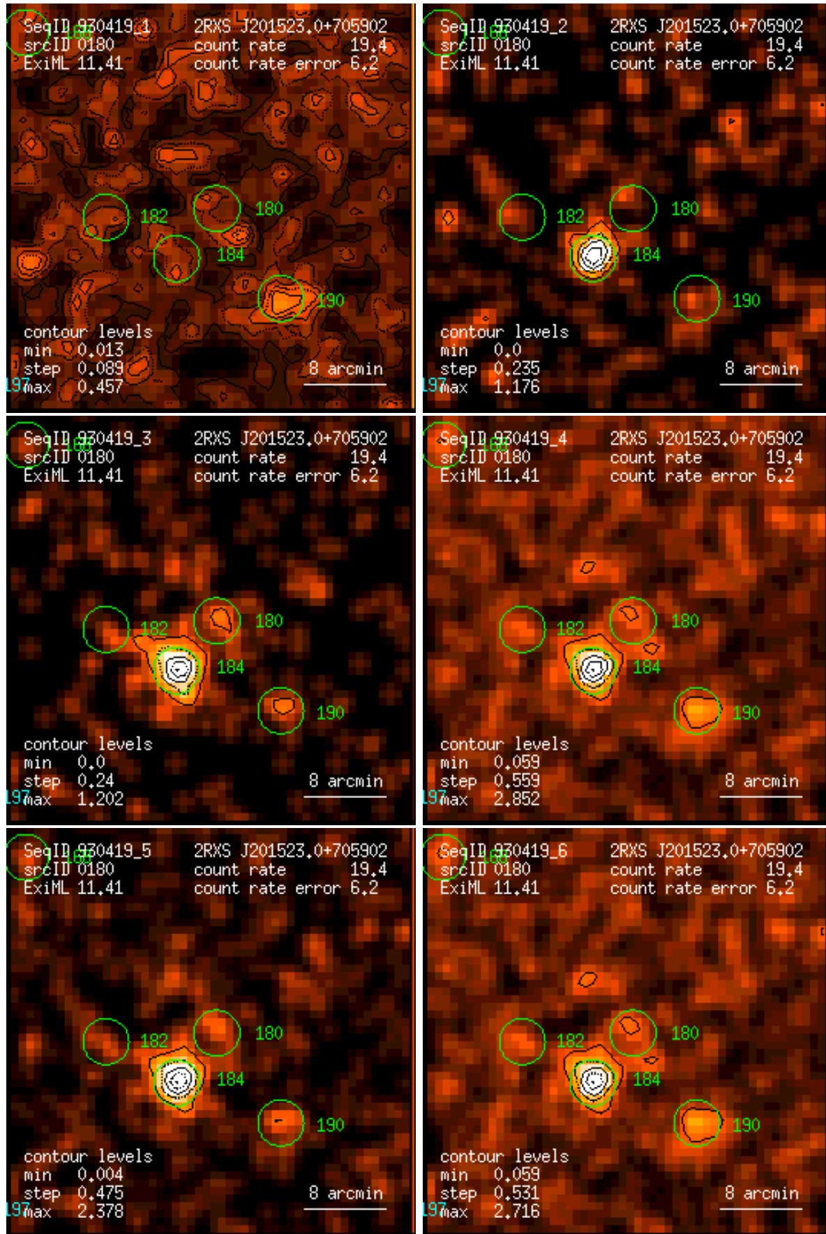
Figure 180: RASS 930419: detection 0180: band rate images, Gaussian filter: (1) PSPC channels 11 – 41, (2) 52 – 90, (3) 91 – 201, (4) 11 – 235, (5) 52 – 201, (6) 11 – 201. Broad band rates in counts/ks. Band rate contour levels in counts/ks/arcmin 2 .
