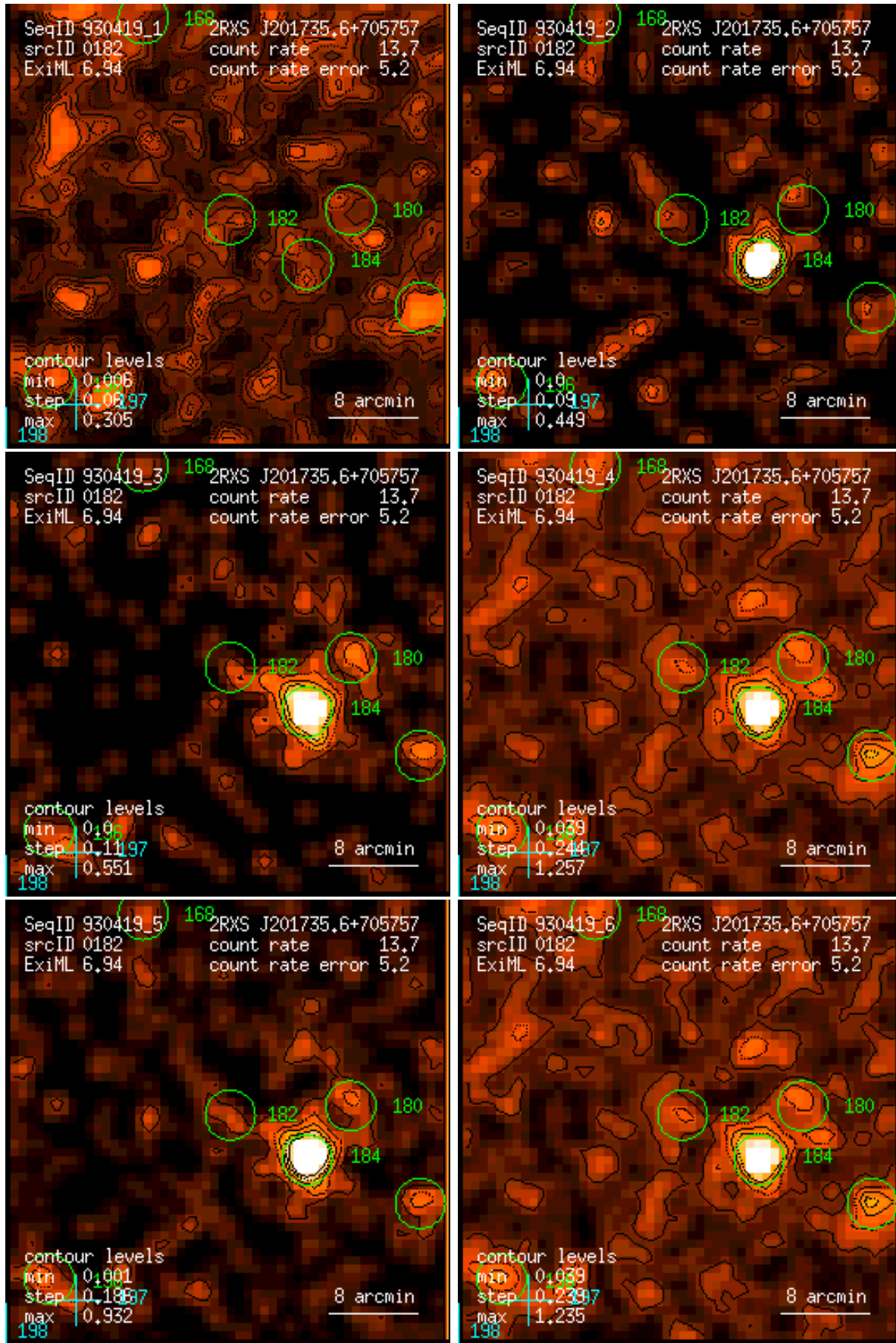
Figure 182: RASS 930419: detection 0182: band rate images, Gaussian filter: (1) PSPC channels 11 – 41, (2) 52 – 90, (3) 91 – 201, (4) 11 – 235, (5) 52 – 201, (6) 11 – 201. Broad band rates in counts/ks. Band rate contour levels in counts/ks/arcmin 2 .
