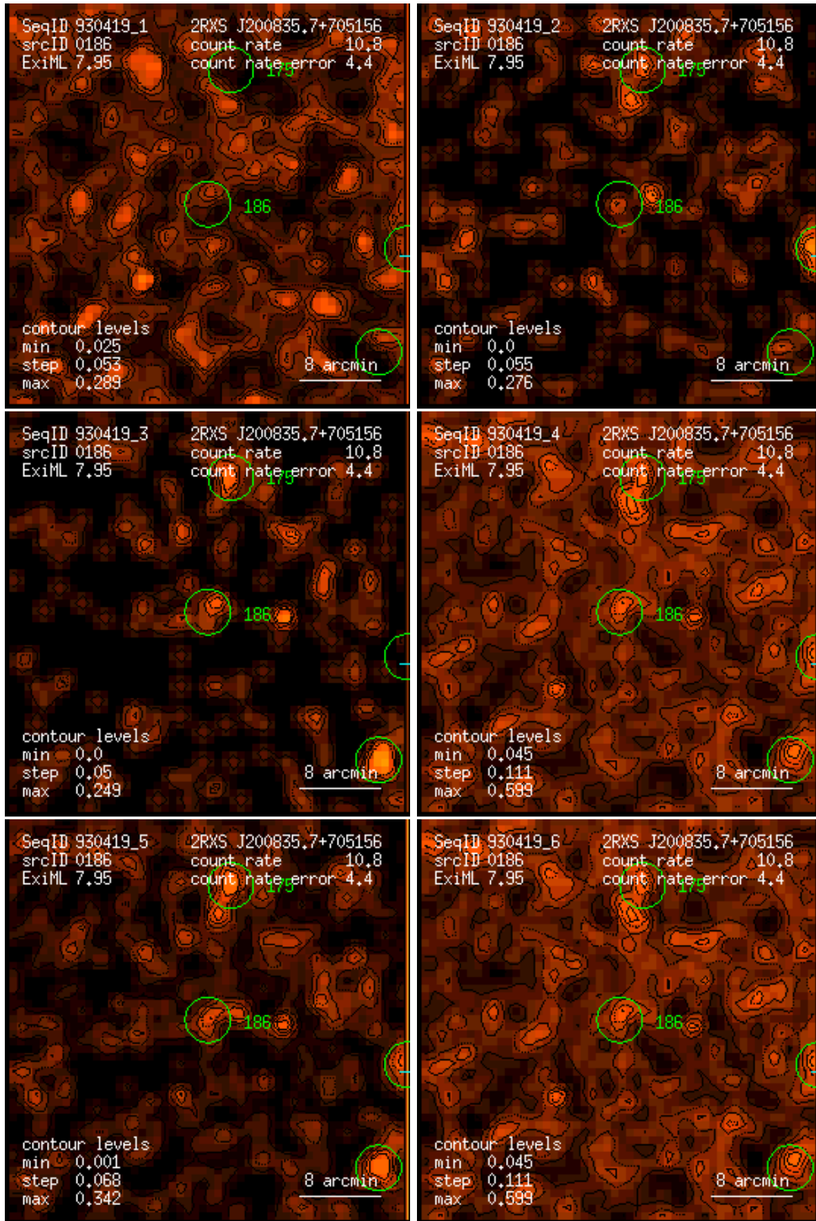
Figure 186: RASS 930419: detection 0186: band rate images, Gaussian filter: (1) PSPC channels 11 – 41, (2) 52 – 90, (3) 91 – 201, (4) 11 – 235, (5) 52 – 201, (6) 11 – 201. Broad band rates in counts/ks. Band rate contour levels in counts/ks/arcmin 2 .
