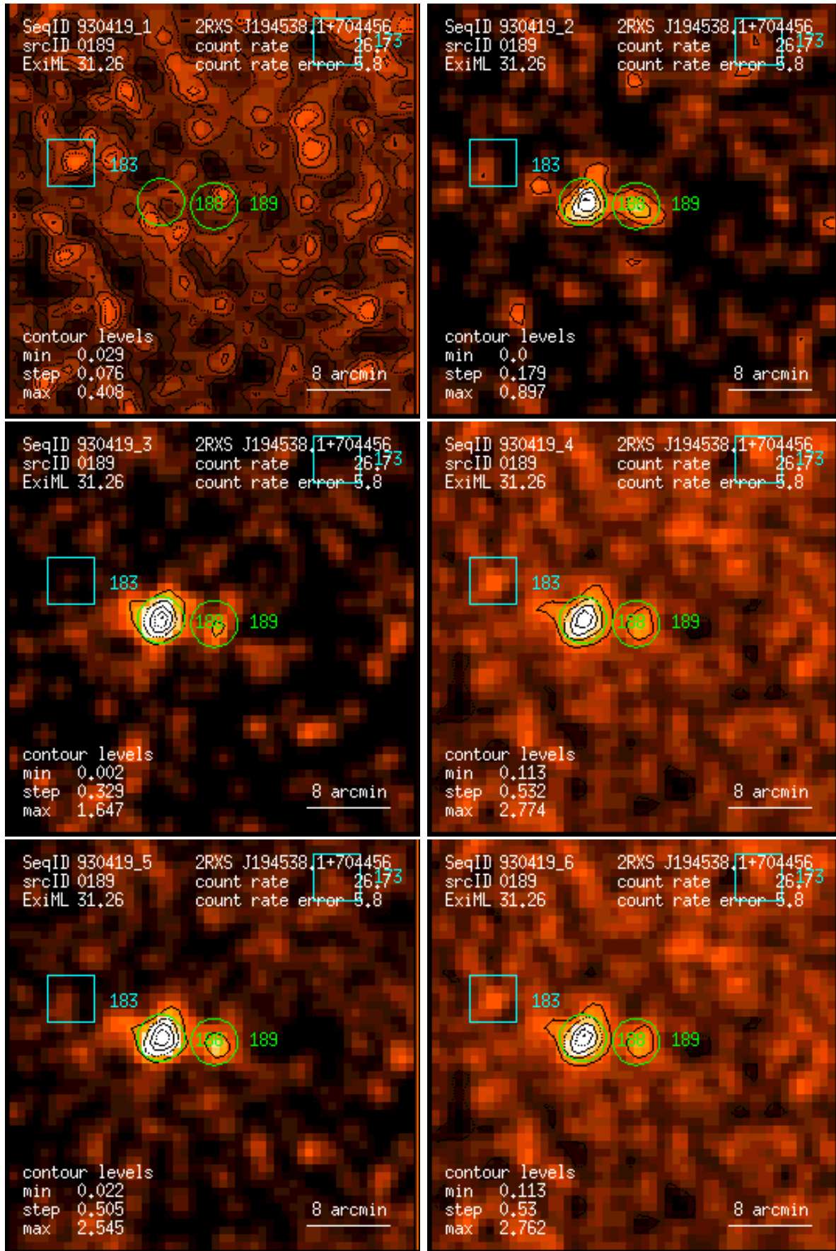
Figure 189: RASS 930419: detection 0189: band rate images, Gaussian filter: (1) PSPC channels 11 – 41, (2) 52 – 90, (3) 91 – 201, (4) 11 – 235, (5) 52 – 201, (6) 11 – 201. Broad band rates in counts/ks. Band rate contour levels in counts/ks/arcmin 2 .
