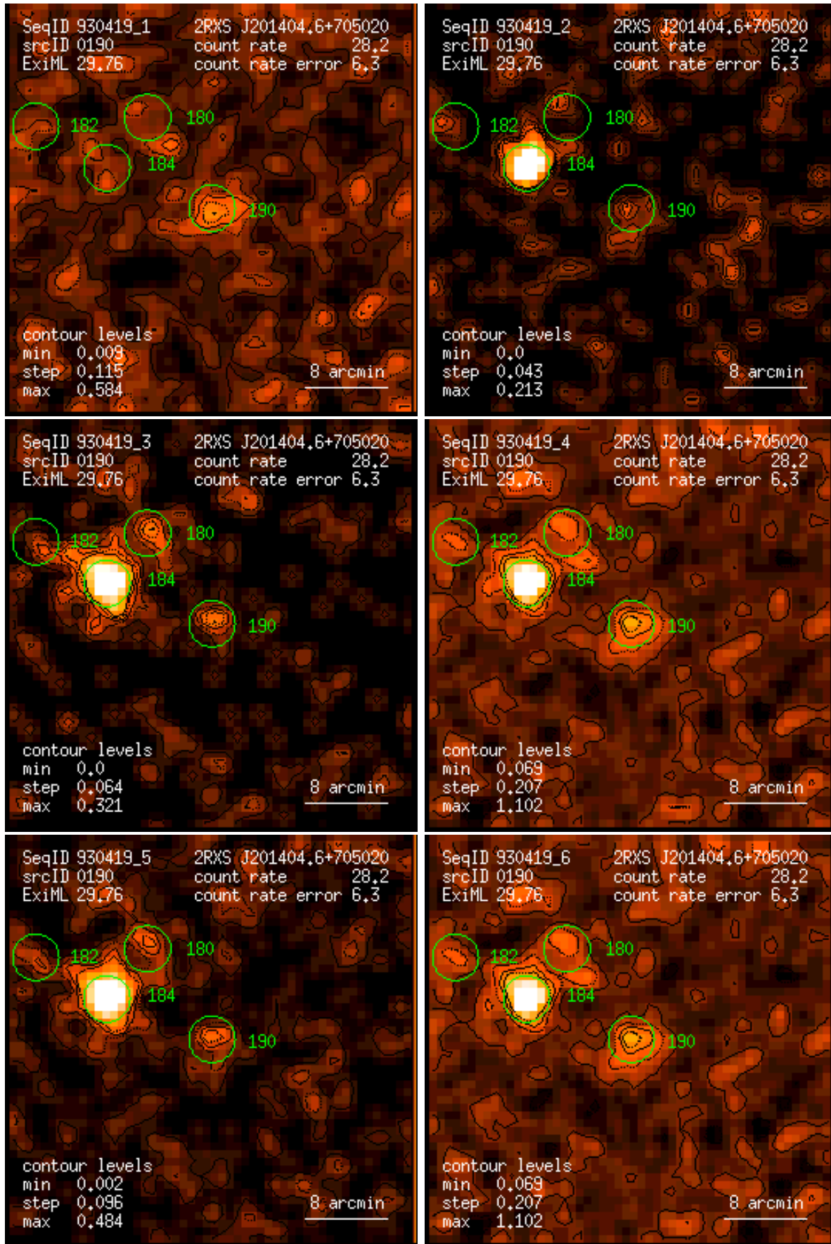
Figure 190: RASS 930419: detection 0190: band rate images, Gaussian filter: (1) PSPC channels 11 – 41, (2) 52 – 90, (3) 91 – 201, (4) 11 – 235, (5) 52 – 201, (6) 11 – 201. Broad band rates in counts/ks. Band rate contour levels in counts/ks/arcmin 2 .
