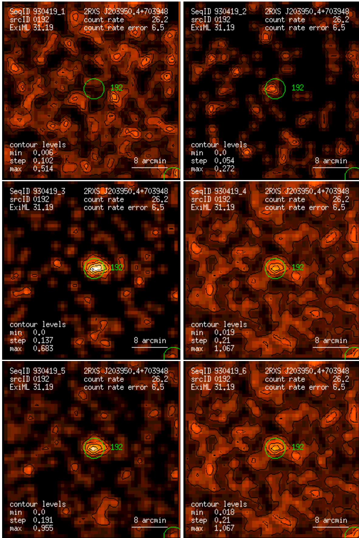
Figure 192: RASS 930419: detection 0192: band rate images, Gaussian filter: (1) PSPC channels 11 – 41, (2) 52 – 90, (3) 91 – 201, (4) 11 – 235, (5) 52 – 201, (6) 11 – 201. Broad band rates in counts/ks. Band rate contour levels in counts/ks/arcmin 2 .
