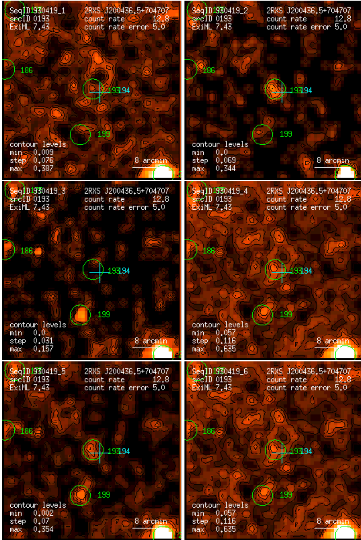
Figure 193: RASS 930419: detection 0193: band rate images, Gaussian filter: (1) PSPC channels 11 – 41, (2) 52 – 90, (3) 91 – 201, (4) 11 – 235, (5) 52 – 201, (6) 11 – 201. Broad band rates in counts/ks. Band rate contour levels in counts/ks/arcmin 2 .
