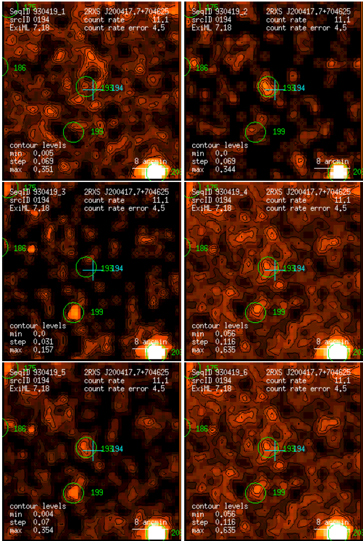
Figure 194: RASS 930419: detection 0194: band rate images, Gaussian filter: (1) PSPC channels 11 – 41, (2) 52 – 90, (3) 91 – 201, (4) 11 – 235, (5) 52 – 201, (6) 11 – 201. Broad band rates in counts/ks. Band rate contour levels in counts/ks/arcmin 2 .
