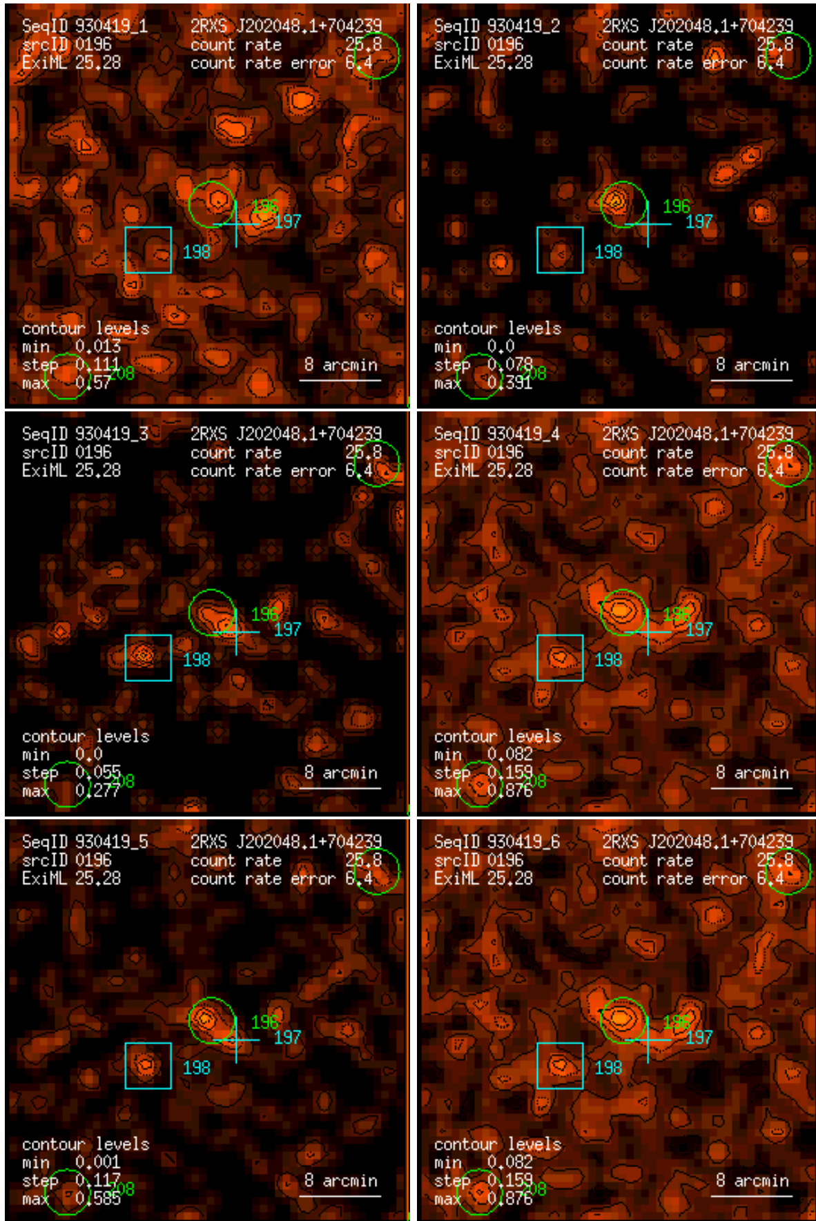
Figure 196: RASS 930419: detection 0196: band rate images, Gaussian filter: (1) PSPC channels 11 – 41, (2) 52 – 90, (3) 91 – 201, (4) 11 – 235, (5) 52 – 201, (6) 11 – 201. Broad band rates in counts/ks. Band rate contour levels in counts/ks/arcmin 2 .
