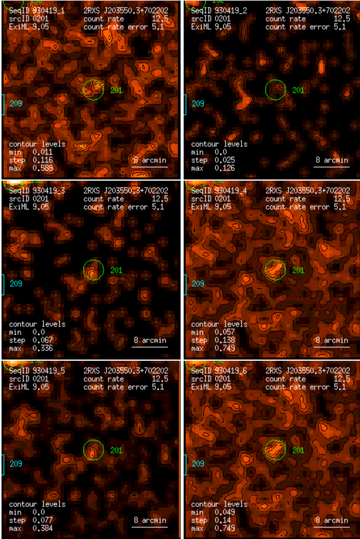
Figure 201: RASS 930419: detection 0201: band rate images, Gaussian filter: (1) PSPC channels 11 – 41, (2) 52 – 90, (3) 91 – 201, (4) 11 – 235, (5) 52 – 201, (6) 11 – 201. Broad band rates in counts/ks. Band rate contour levels in counts/ks/arcmin 2 .
