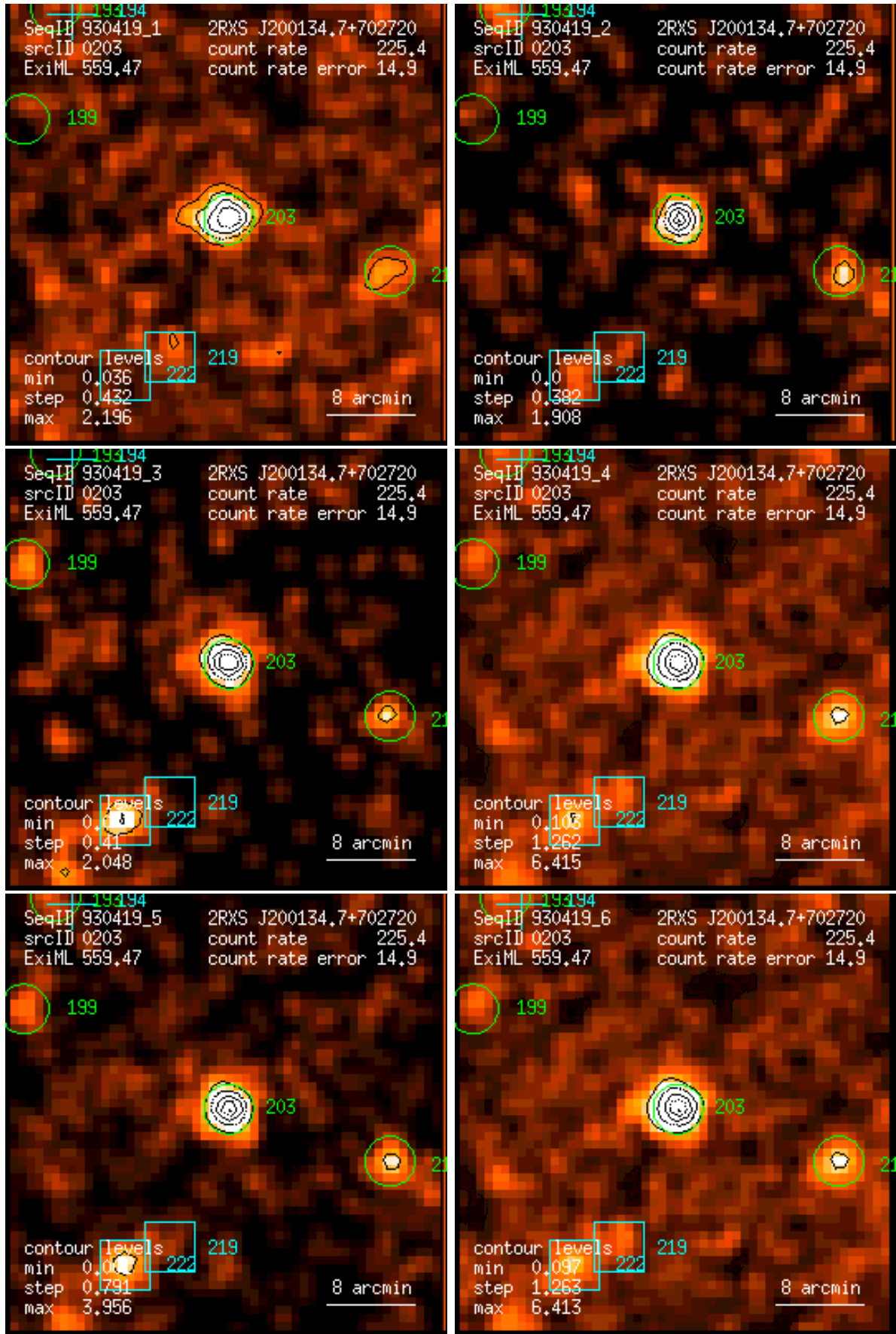
Figure 203: RASS 930419: detection 0203: band rate images, Gaussian filter: (1) PSPC channels 11 – 41, (2) 52 – 90, (3) 91 – 201, (4) 11 – 235, (5) 52 – 201, (6) 11 – 201. Broad band rates in counts/ks. Band rate contour levels in counts/ks/arcmin 2 .
