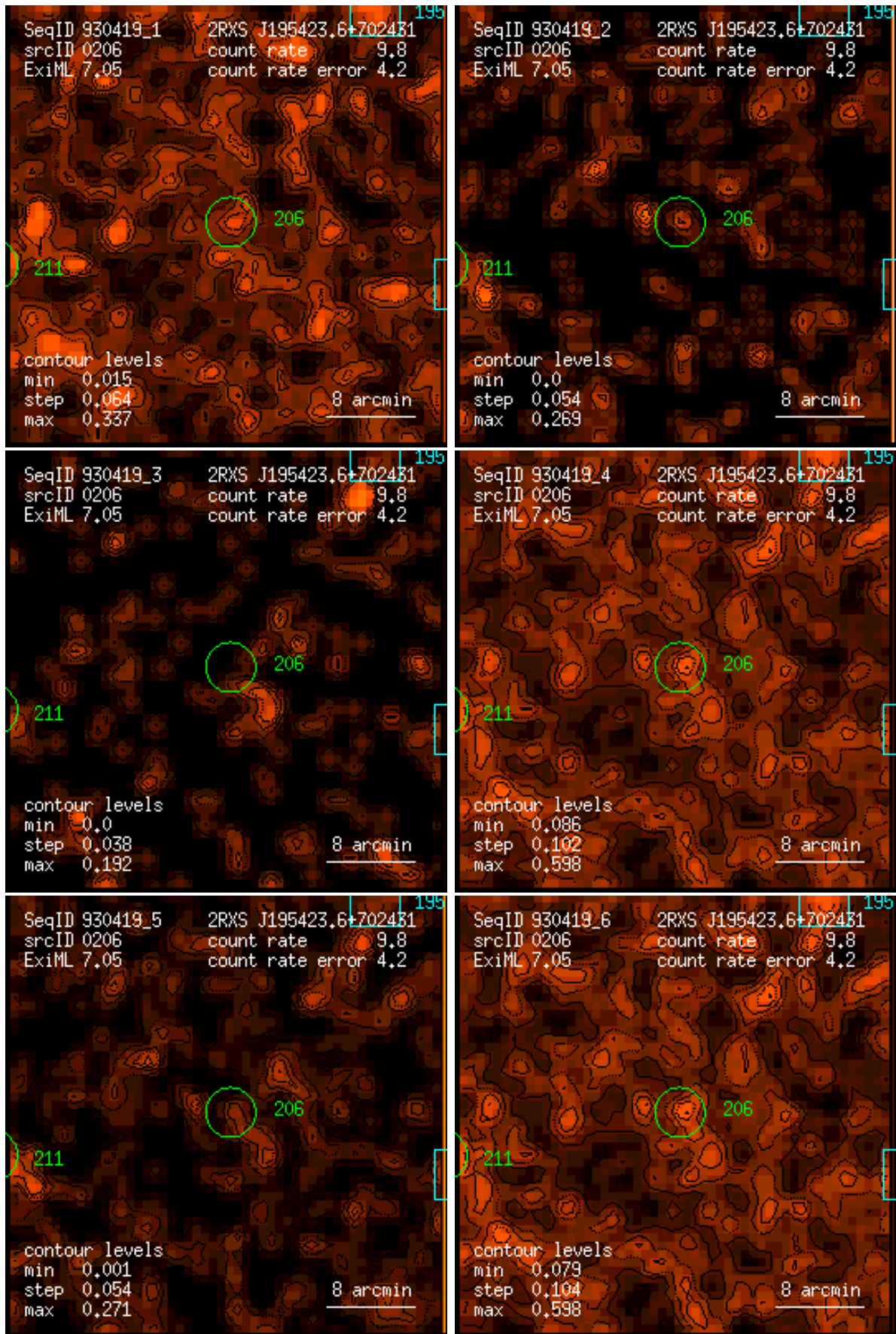
Figure 206: RASS 930419: detection 0206: band rate images, Gaussian filter: (1) PSPC channels 11 – 41, (2) 52 – 90, (3) 91 – 201, (4) 11 – 235, (5) 52 – 201, (6) 11 – 201. Broad band rates in counts/ks. Band rate contour levels in counts/ks/arcmin 2 .
