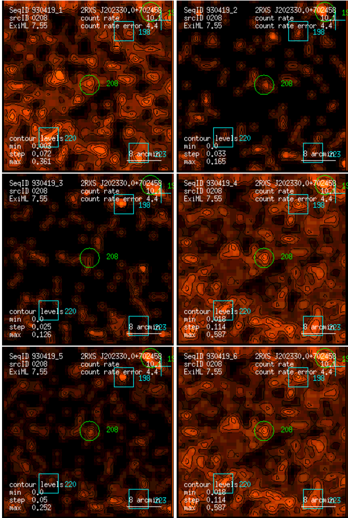
Figure 208: RASS 930419: detection 0208: band rate images, Gaussian filter: (1) PSPC channels 11 – 41, (2) 52 – 90, (3) 91 – 201, (4) 11 – 235, (5) 52 – 201, (6) 11 – 201. Broad band rates in counts/ks. Band rate contour levels in counts/ks/arcmin 2 .
