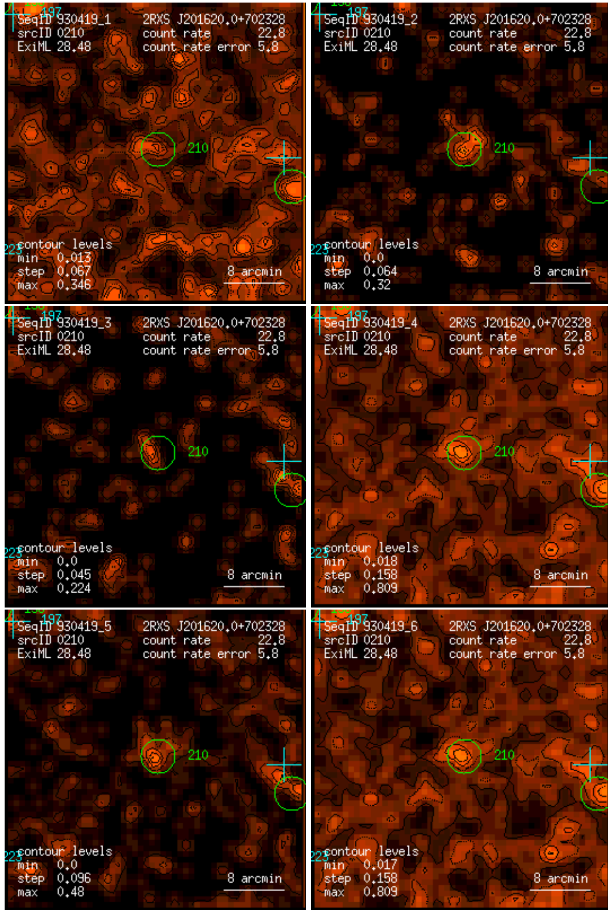
Figure 210: RASS 930419: detection 0210: band rate images, Gaussian filter: (1) PSPC channels 11 – 41, (2) 52 – 90, (3) 91 – 201, (4) 11 – 235, (5) 52 – 201, (6) 11 – 201. Broad band rates in counts/ks. Band rate contour levels in counts/ks/arcmin 2 .
