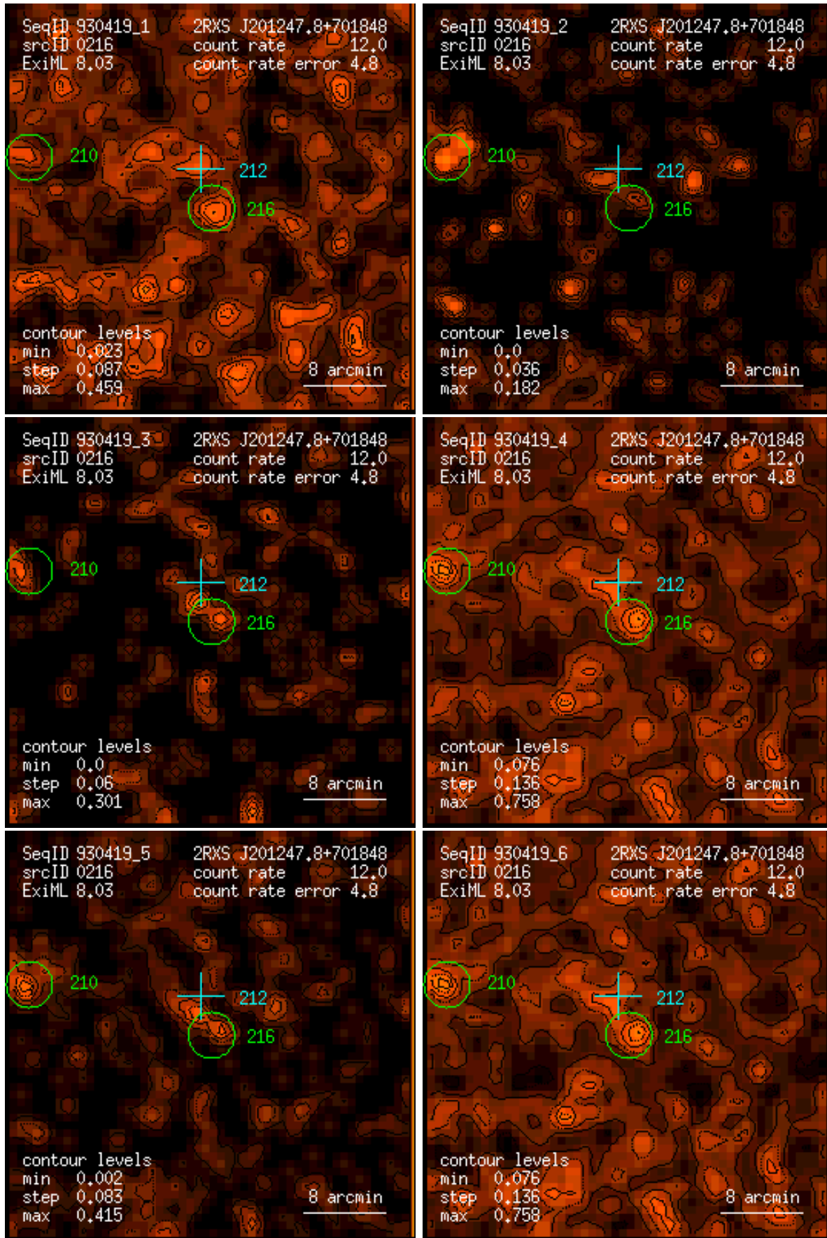
Figure 216: RASS 930419: detection 0216: band rate images, Gaussian filter: (1) PSPC channels 11 – 41, (2) 52 – 90, (3) 91 – 201, (4) 11 – 235, (5) 52 – 201, (6) 11 – 201. Broad band rates in counts/ks. Band rate contour levels in counts/ks/arcmin 2 .
