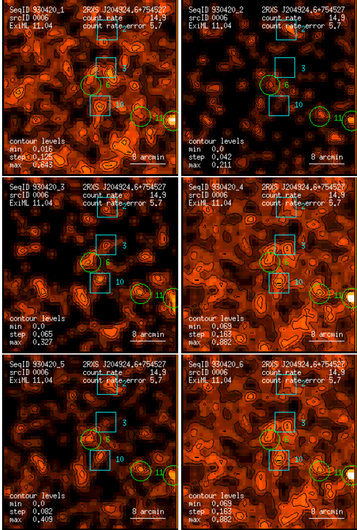
Figure 6: RASS 930420: detection 0006: band rate images, Gaussian filter: (1) PSPC channels 11 – 41, (2) 52 – 90, (3) 91 – 201, (4) 11 – 235, (5) 52 – 201, (6) 11 – 201. Broad band rates in counts/ks. Band rate contour levels in counts/ks/arcmin 2 .
