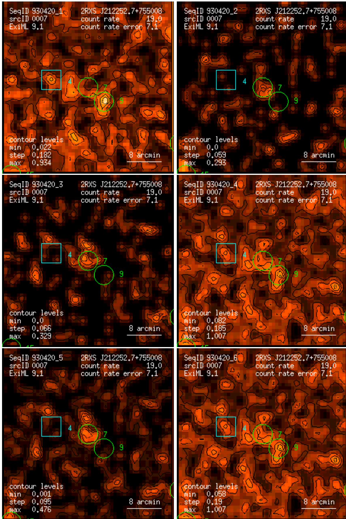
Figure 7: RASS 930420: detection 0007: band rate images, Gaussian filter: (1) PSPC channels 11 – 41, (2) 52 – 90, (3) 91 – 201, (4) 11 – 235, (5) 52 – 201, (6) 11 – 201. Broad band rates in counts/ks. Band rate contour levels in counts/ks/arcmin 2 .
