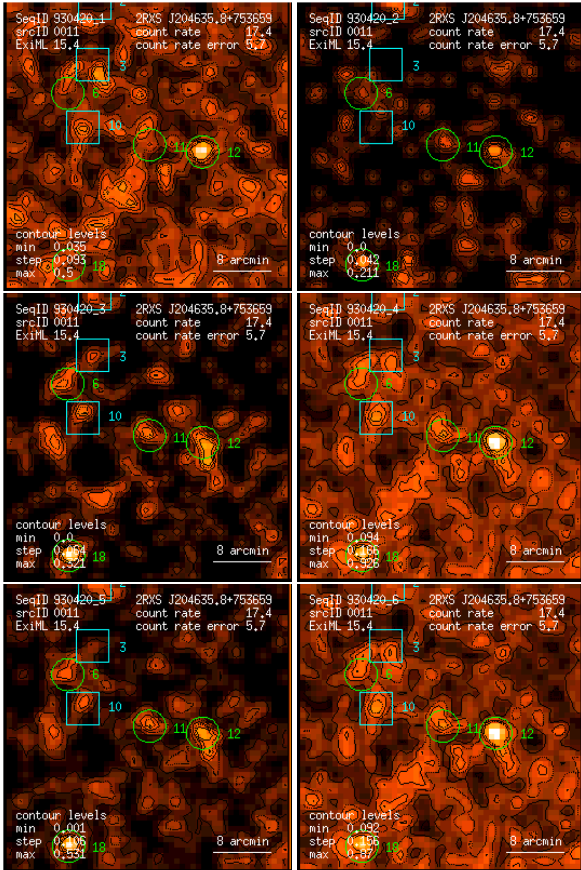
Figure 11: RASS 930420: detection 0011: band rate images, Gaussian filter: (1) PSPC channels 11 – 41, (2) 52 – 90, (3) 91 – 201, (4) 11 – 235, (5) 52 – 201, (6) 11 – 201. Broad band rates in counts/ks. Band rate contour levels in counts/ks/arcmin 2 .
