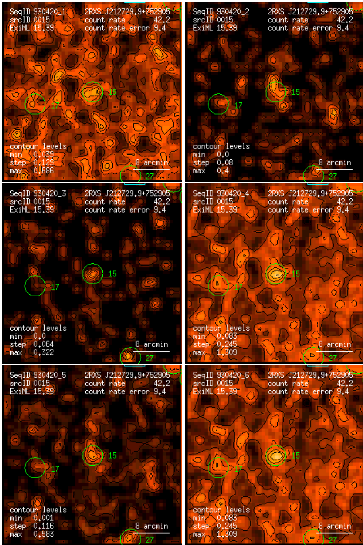
Figure 15: RASS 930420: detection 0015: band rate images, Gaussian filter: (1) PSPC channels 11 – 41, (2) 52 – 90, (3) 91 – 201, (4) 11 – 235, (5) 52 – 201, (6) 11 – 201. Broad band rates in counts/ks. Band rate contour levels in counts/ks/arcmin 2 .
