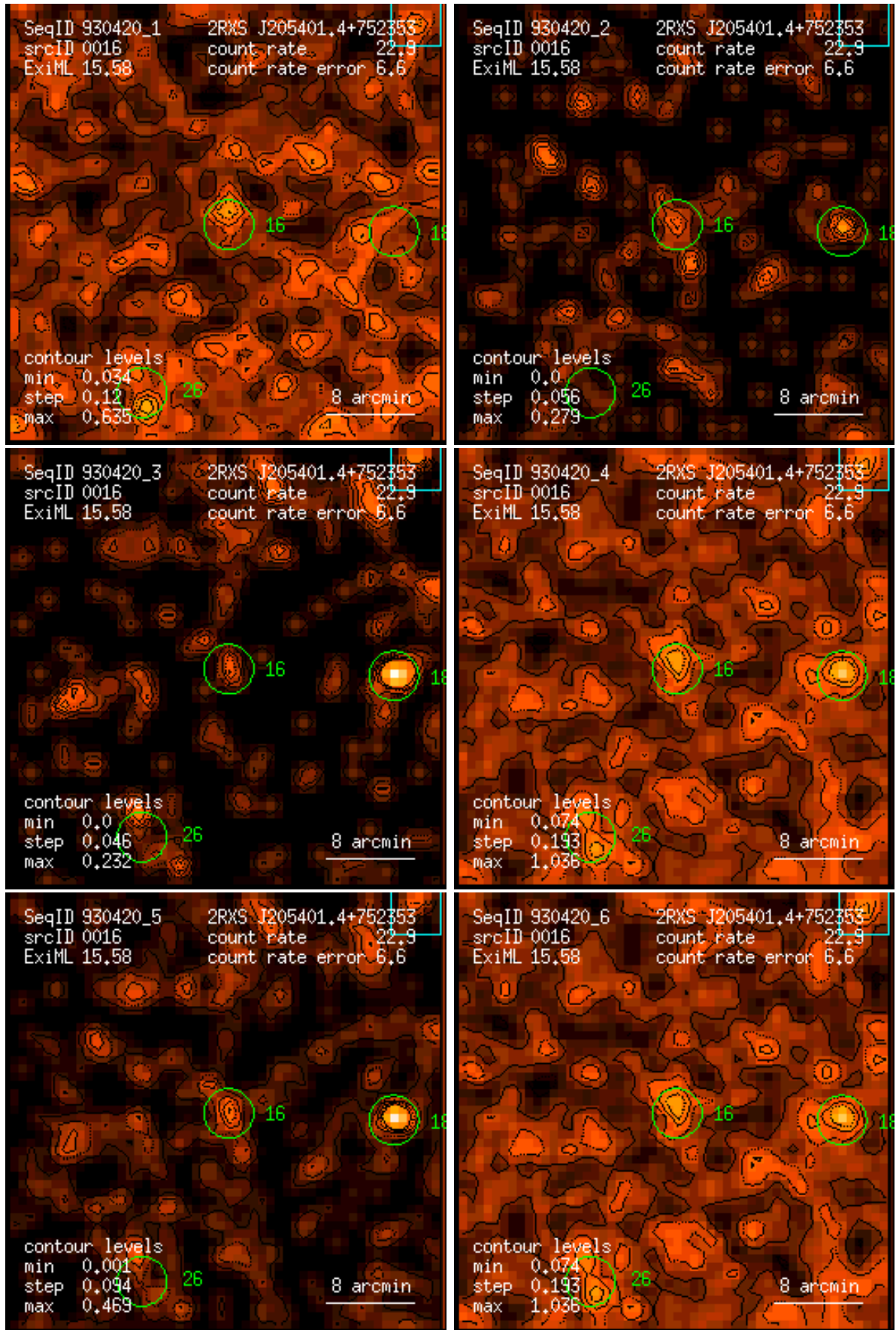
Figure 16: RASS 930420: detection 0016: band rate images, Gaussian filter: (1) PSPC channels 11 – 41, (2) 52 – 90, (3) 91 – 201, (4) 11 – 235, (5) 52 – 201, (6) 11 – 201. Broad band rates in counts/ks. Band rate contour levels in counts/ks/arcmin 2 .
