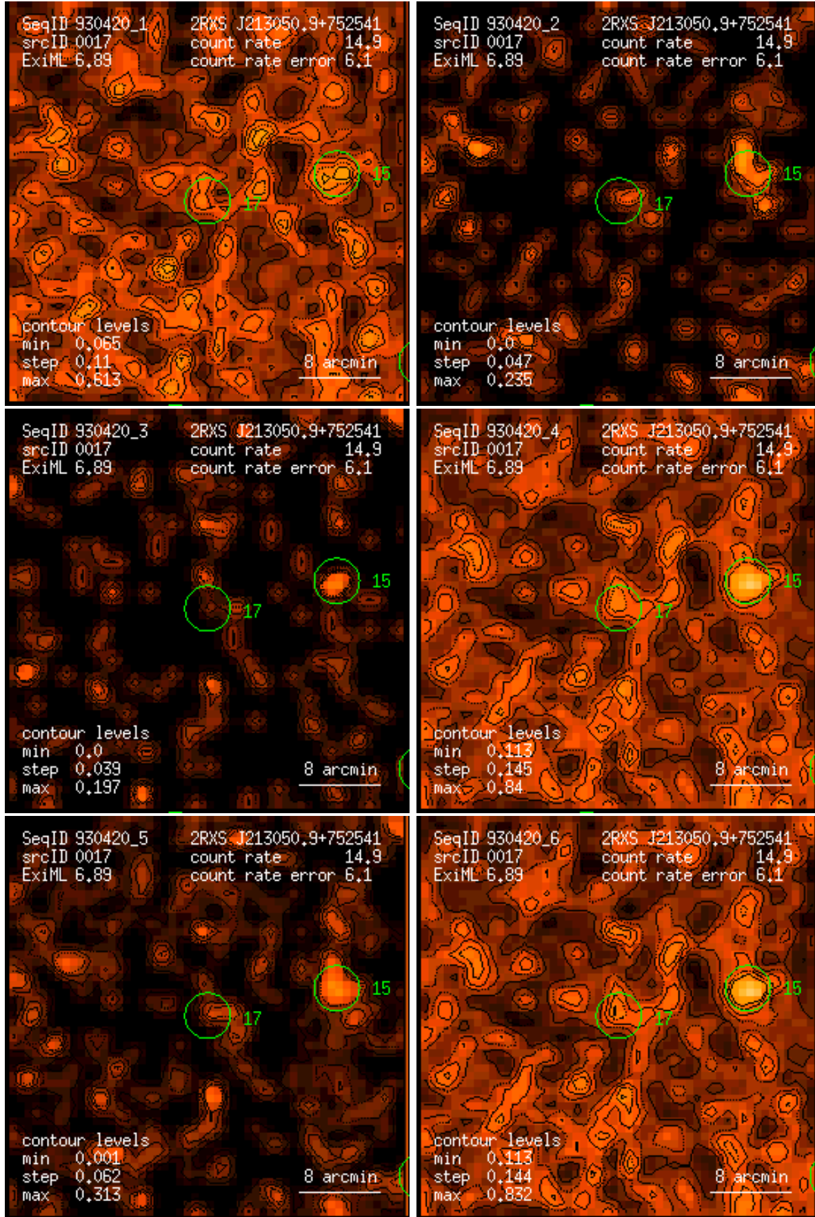
Figure 17: RASS 930420: detection 0017: band rate images, Gaussian filter: (1) PSPC channels 11 – 41, (2) 52 – 90, (3) 91 – 201, (4) 11 – 235, (5) 52 – 201, (6) 11 – 201. Broad band rates in counts/ks. Band rate contour levels in counts/ks/arcmin 2 .
