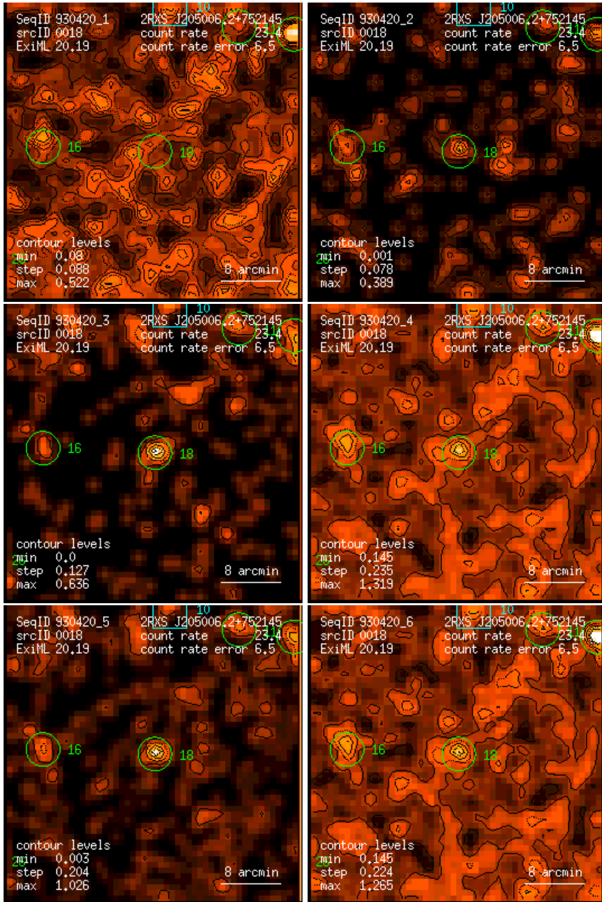
Figure 18: RASS 930420: detection 0018: band rate images, Gaussian filter: (1) PSPC channels 11 – 41, (2) 52 – 90, (3) 91 – 201, (4) 11 – 235, (5) 52 – 201, (6) 11 – 201. Broad band rates in counts/ks. Band rate contour levels in counts/ks/arcmin 2 .
