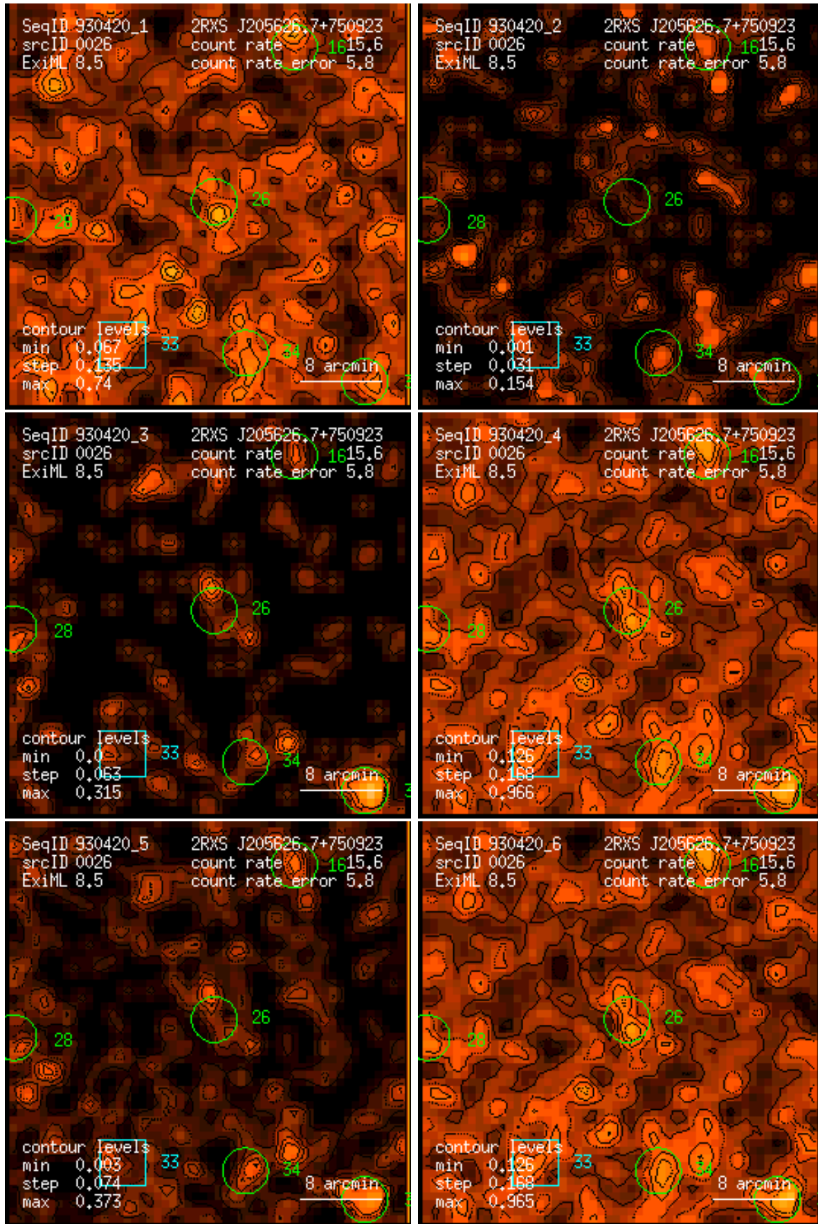
Figure 26: RASS 930420: detection 0026: band rate images, Gaussian filter: (1) PSPC channels 11 – 41, (2) 52 – 90, (3) 91 – 201, (4) 11 – 235, (5) 52 – 201, (6) 11 – 201. Broad band rates in counts/ks. Band rate contour levels in counts/ks/arcmin 2 .
