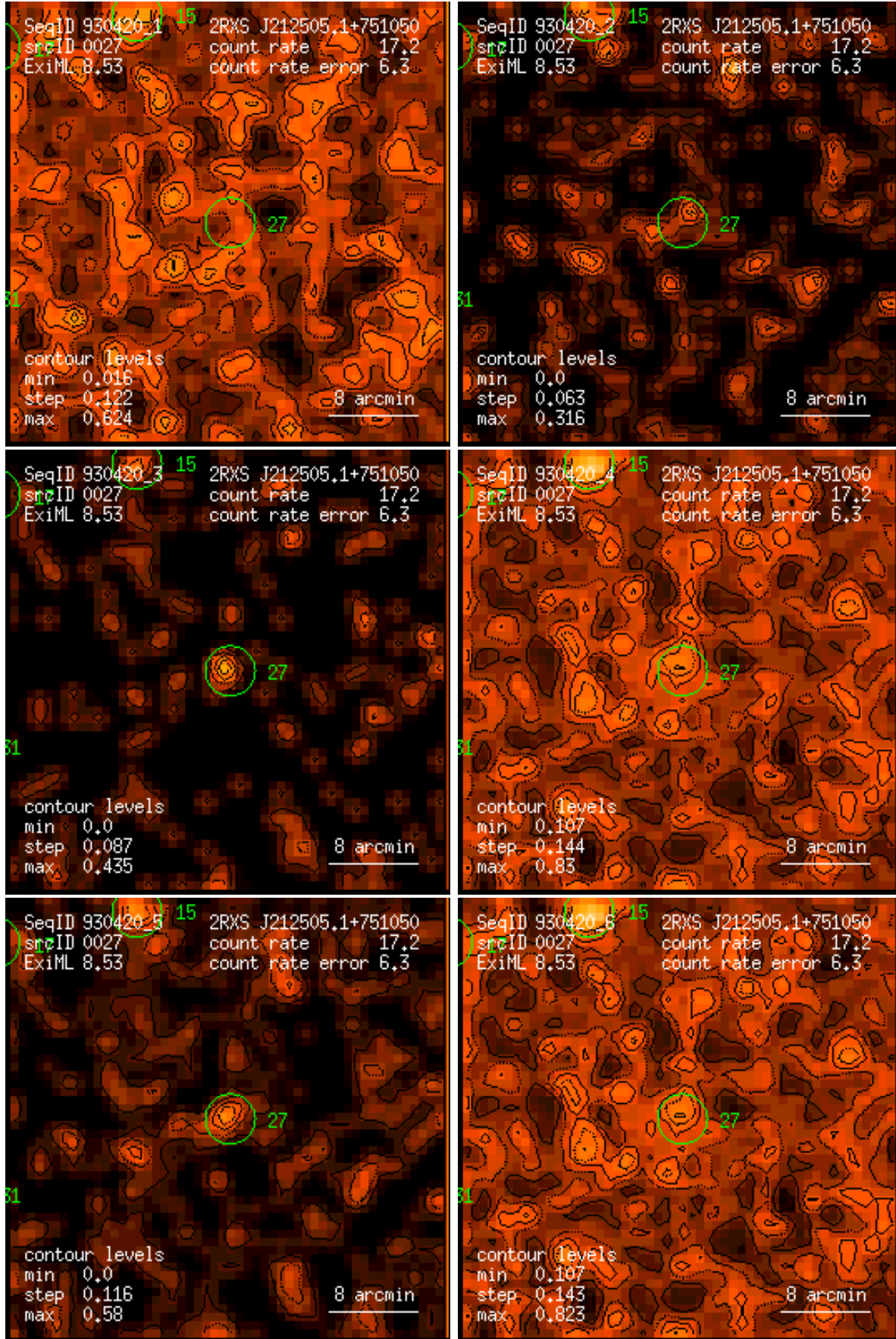
Figure 27: RASS 930420: detection 0027: band rate images, Gaussian filter: (1) PSPC channels 11 – 41, (2) 52 – 90, (3) 91 – 201, (4) 11 – 235, (5) 52 – 201, (6) 11 – 201. Broad band rates in counts/ks. Band rate contour levels in counts/ks/arcmin 2 .
