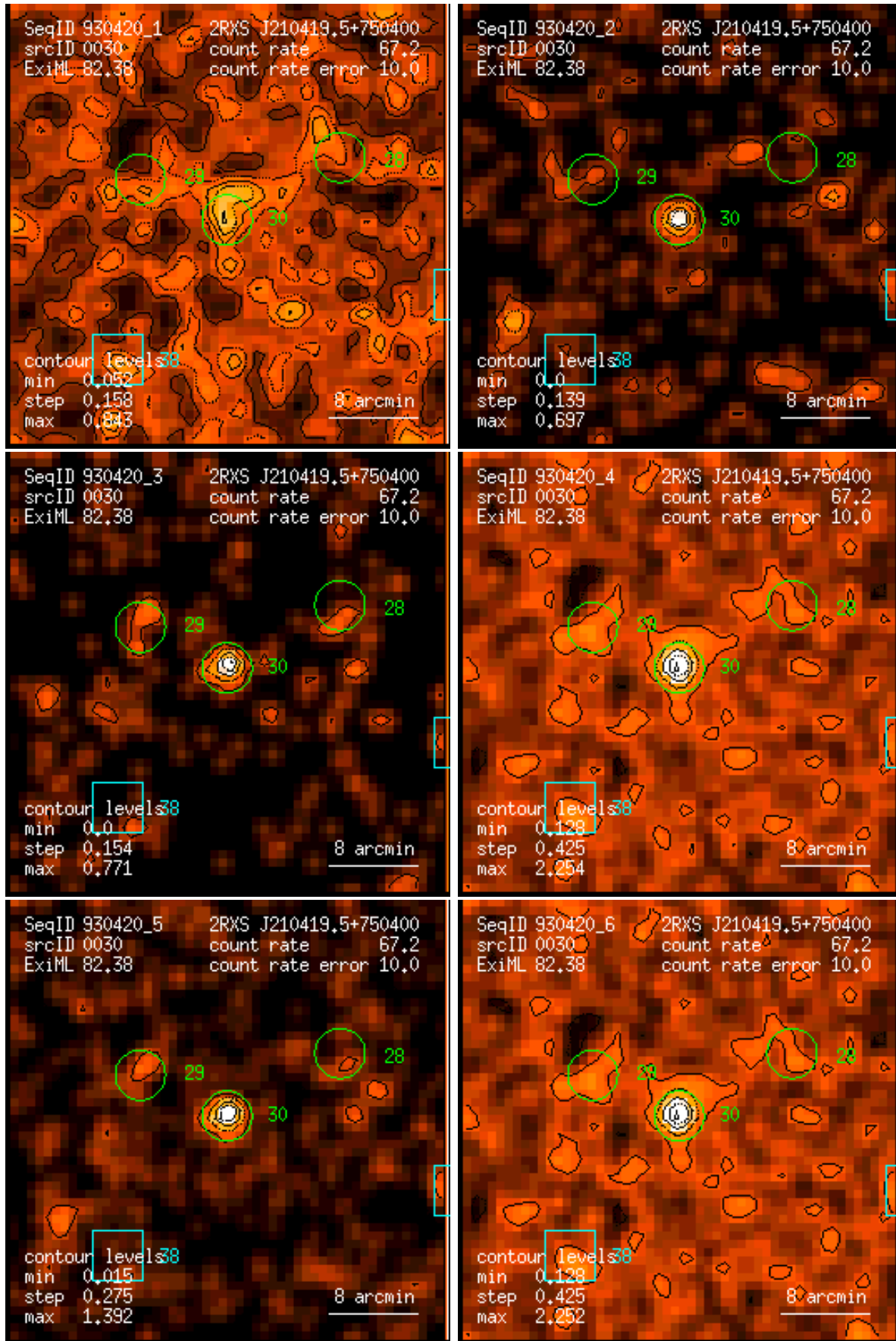
Figure 30: RASS 930420: detection 0030: band rate images, Gaussian filter: (1) PSPC channels 11 – 41, (2) 52 – 90, (3) 91 – 201, (4) 11 – 235, (5) 52 – 201, (6) 11 – 201. Broad band rates in counts/ks. Band rate contour levels in counts/ks/arcmin 2 .
