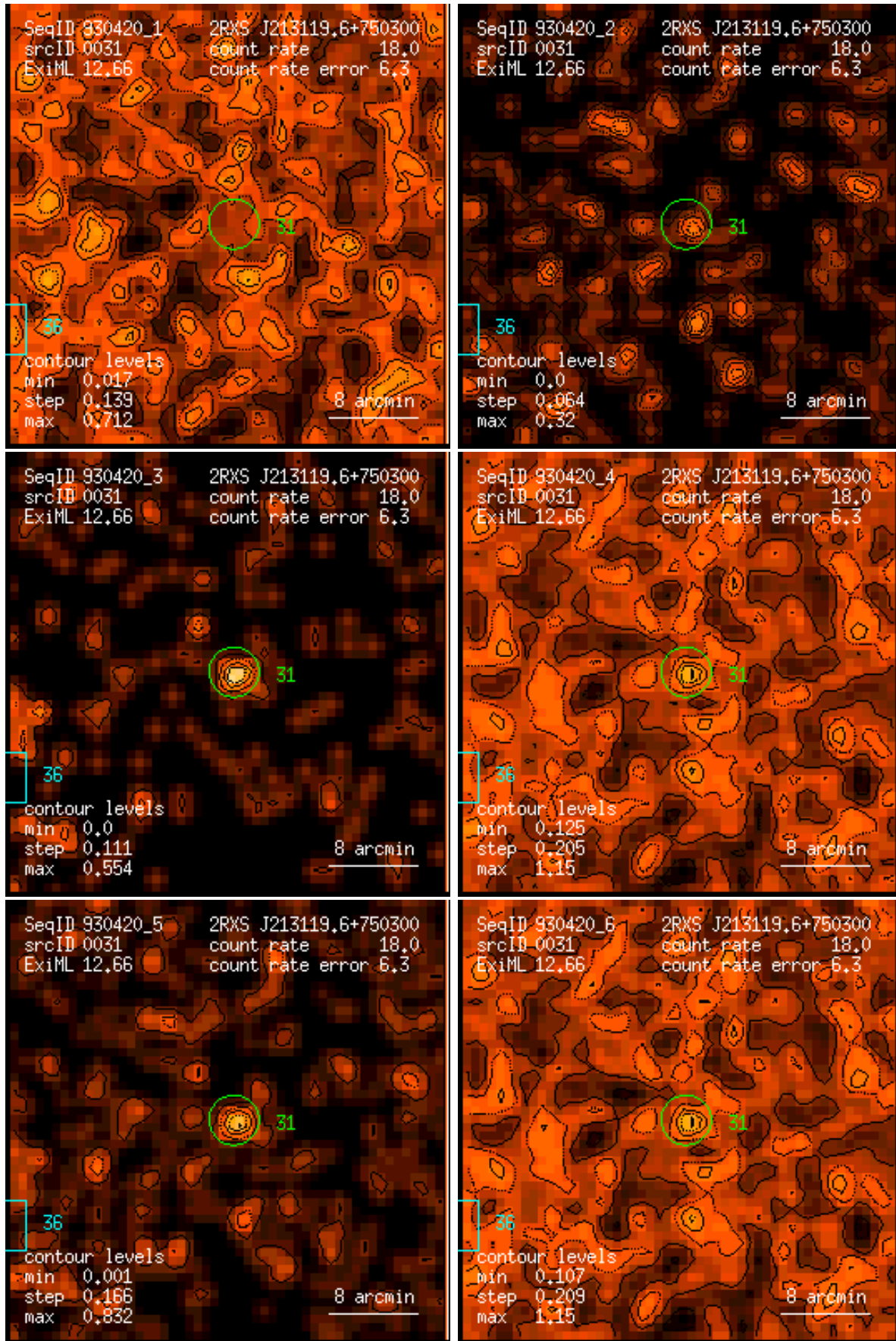
Figure 31: RASS 930420: detection 0031: band rate images, Gaussian filter: (1) PSPC channels 11 – 41, (2) 52 – 90, (3) 91 – 201, (4) 11 – 235, (5) 52 – 201, (6) 11 – 201. Broad band rates in counts/ks. Band rate contour levels in counts/ks/arcmin 2 .
