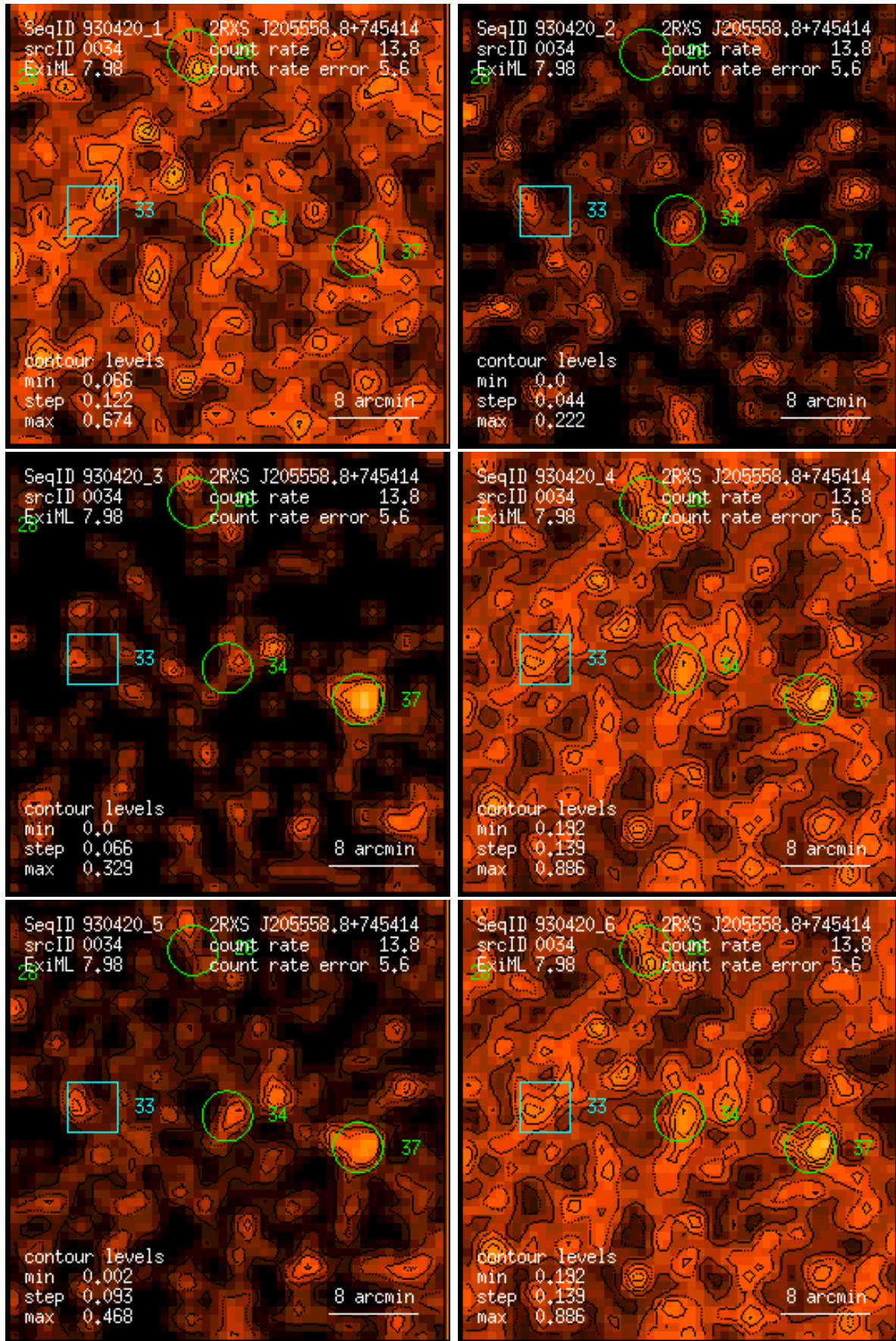
Figure 34: RASS 930420: detection 0034: band rate images, Gaussian filter: (1) PSPC channels 11 – 41, (2) 52 – 90, (3) 91 – 201, (4) 11 – 235, (5) 52 – 201, (6) 11 – 201. Broad band rates in counts/ks. Band rate contour levels in counts/ks/arcmin 2 .
