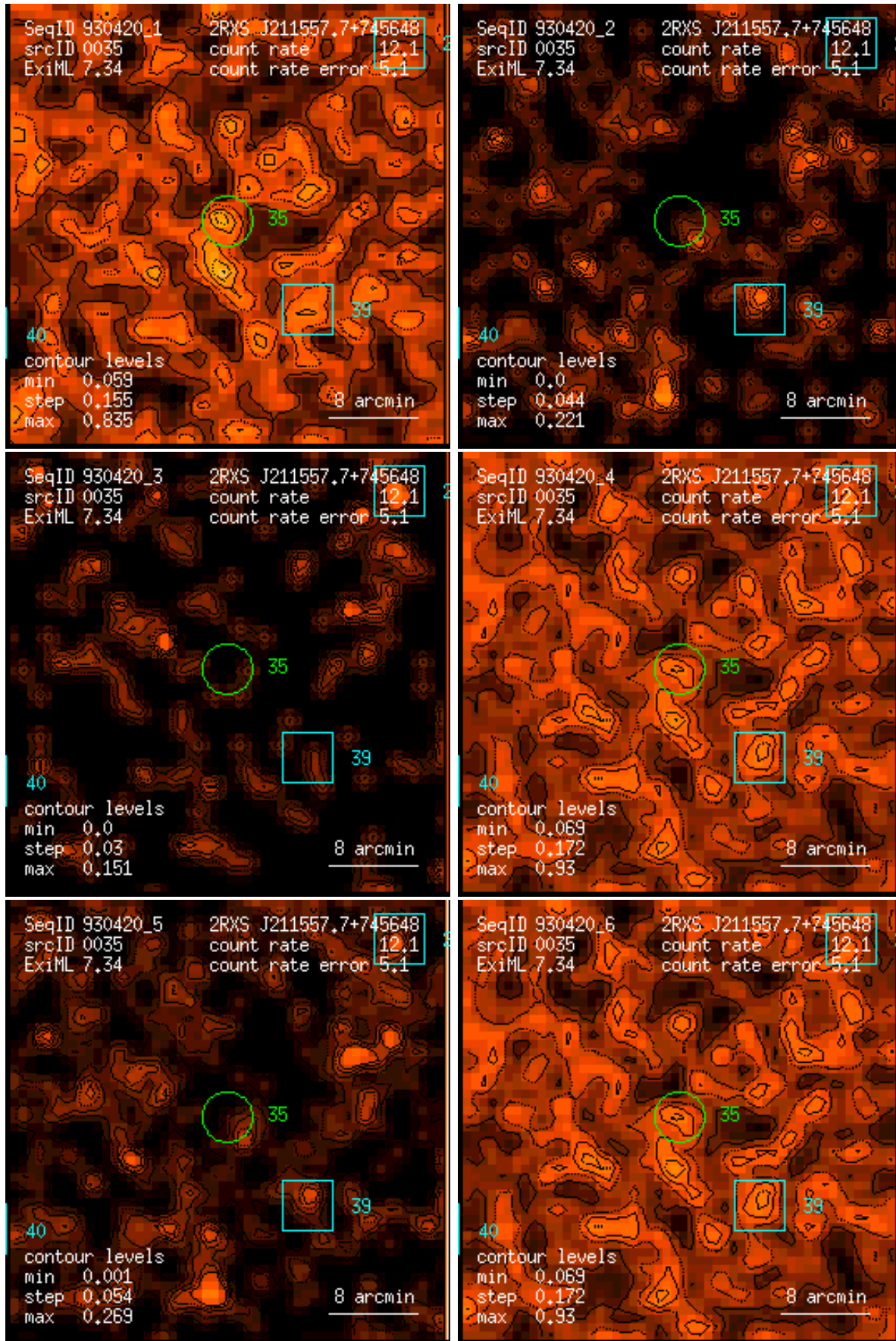
Figure 35: RASS 930420: detection 0035: band rate images, Gaussian filter: (1) PSPC channels 11 – 41, (2) 52 – 90, (3) 91 – 201, (4) 11 – 235, (5) 52 – 201, (6) 11 – 201. Broad band rates in counts/ks. Band rate contour levels in counts/ks/arcmin 2 .
