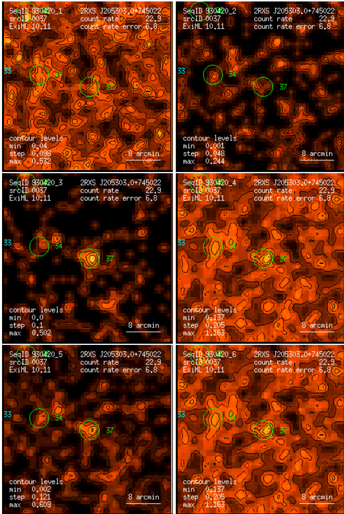
Figure 37: RASS 930420: detection 0037: band rate images, Gaussian filter: (1) PSPC channels 11 – 41, (2) 52 – 90, (3) 91 – 201, (4) 11 – 235, (5) 52 – 201, (6) 11 – 201. Broad band rates in counts/ks. Band rate contour levels in counts/ks/arcmin 2 .
