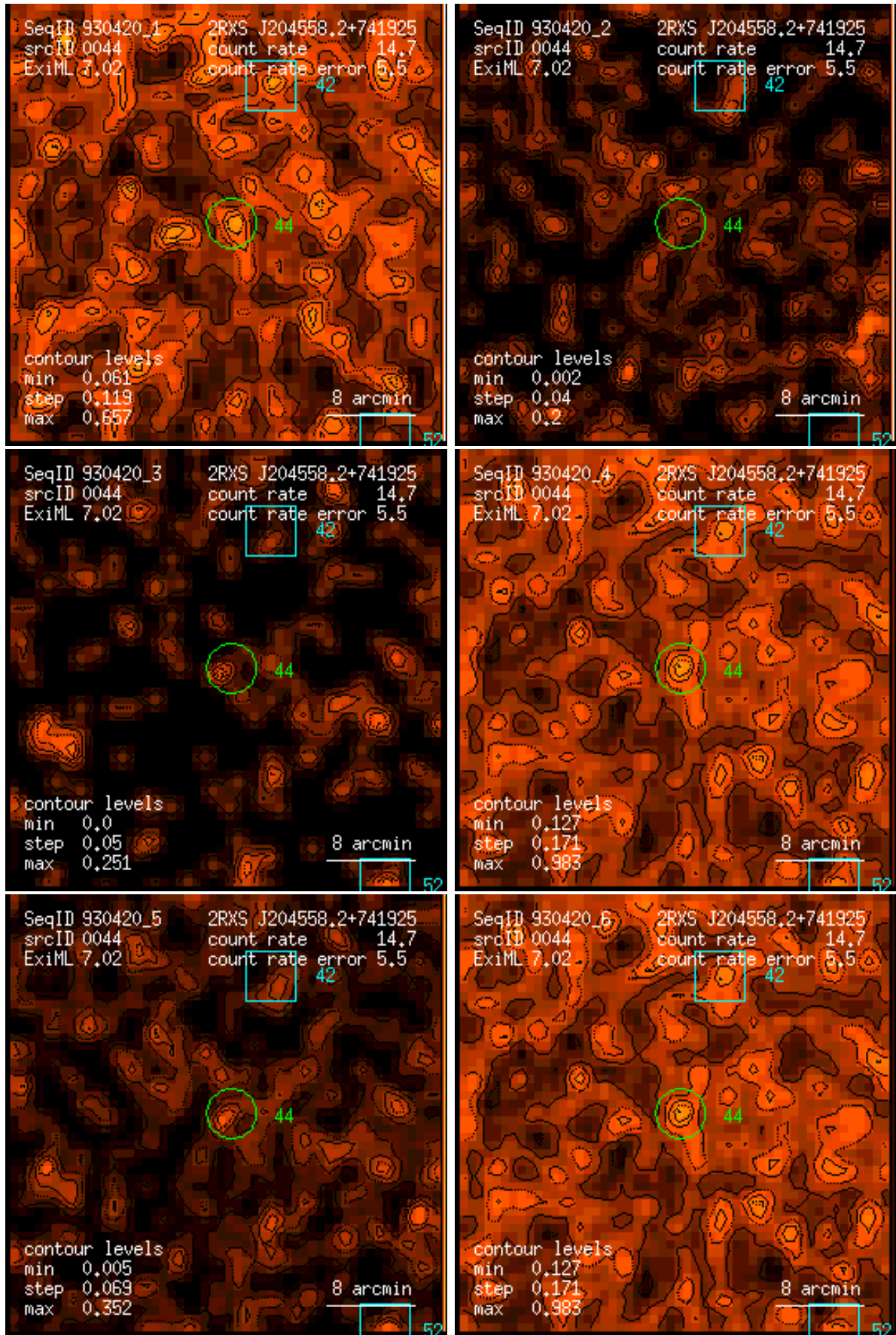
Figure 44: RASS 930420: detection 0044: band rate images, Gaussian filter: (1) PSPC channels 11 – 41, (2) 52 – 90, (3) 91 – 201, (4) 11 – 235, (5) 52 – 201, (6) 11 – 201. Broad band rates in counts/ks. Band rate contour levels in counts/ks/arcmin 2 .
