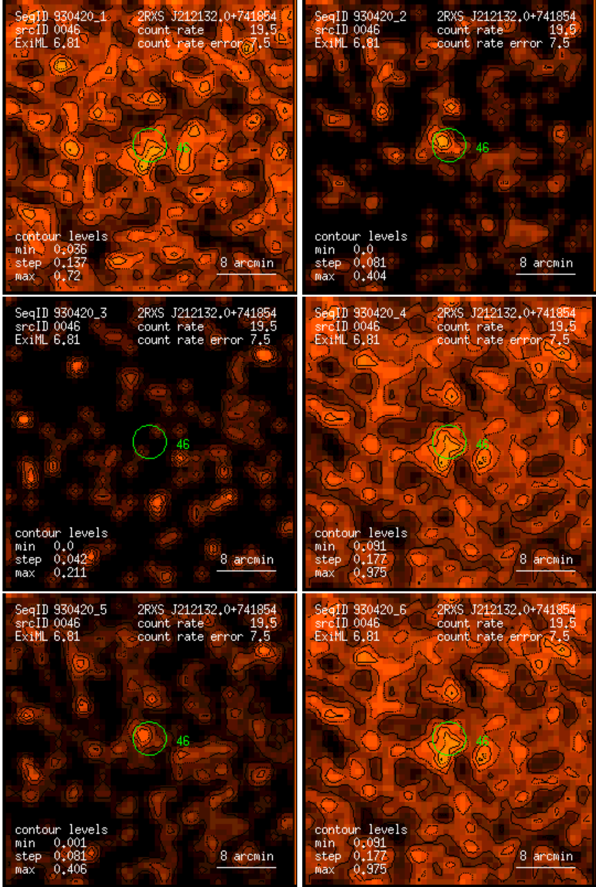
Figure 46: RASS 930420: detection 0046: band rate images, Gaussian filter: (1) PSPC channels 11 – 41, (2) 52 – 90, (3) 91 – 201, (4) 11 – 235, (5) 52 – 201, (6) 11 – 201. Broad band rates in counts/ks. Band rate contour levels in counts/ks/arcmin 2 .
