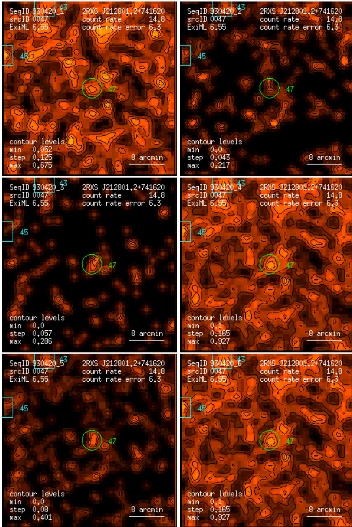
Figure 47: RASS 930420: detection 0047: band rate images, Gaussian filter: (1) PSPC channels 11 – 41, (2) 52 – 90, (3) 91 – 201, (4) 11 – 235, (5) 52 – 201, (6) 11 – 201. Broad band rates in counts/ks. Band rate contour levels in counts/ks/arcmin 2 .
