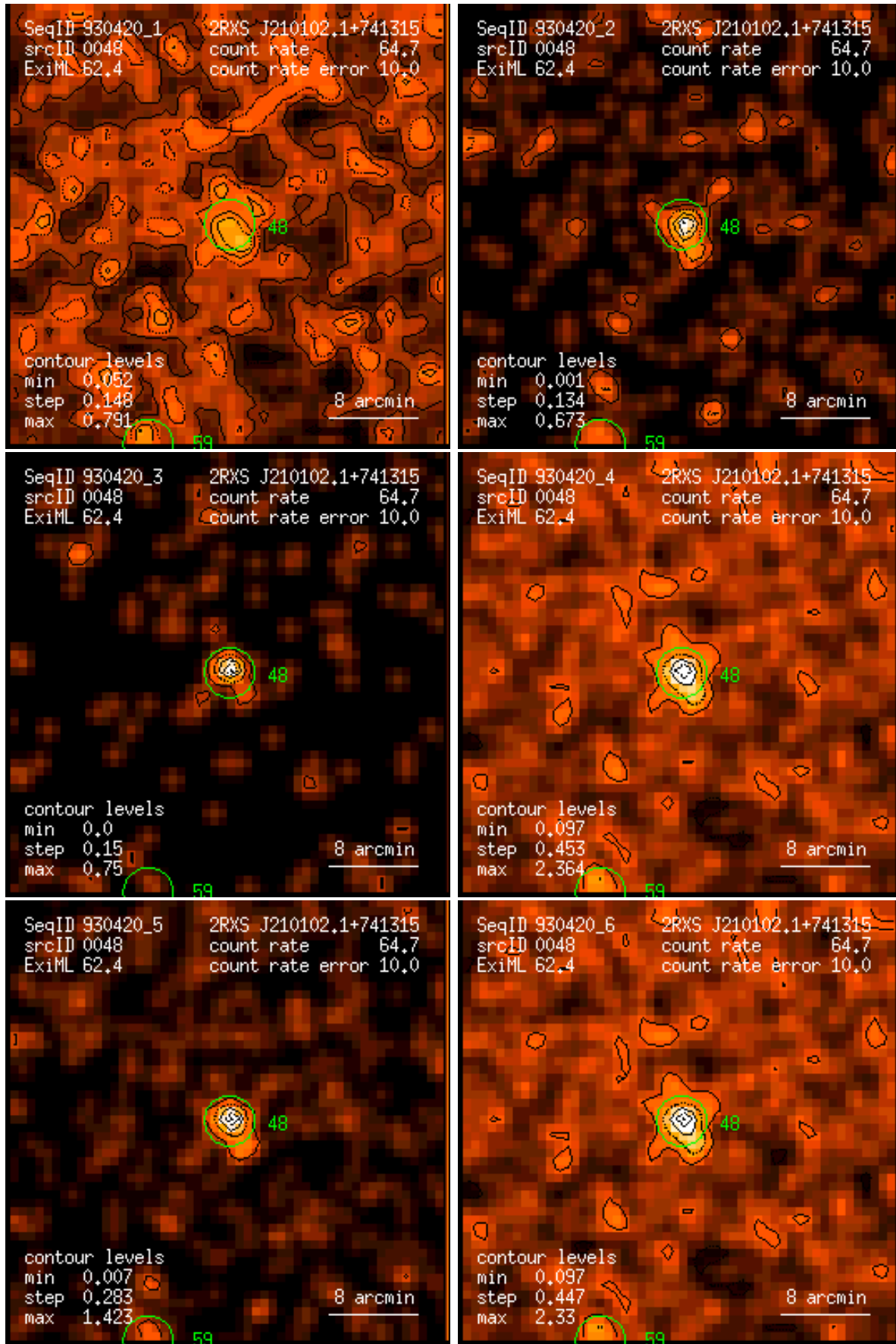
Figure 48: RASS 930420: detection 0048: band rate images, Gaussian filter: (1) PSPC channels 11 – 41, (2) 52 – 90, (3) 91 – 201, (4) 11 – 235, (5) 52 – 201, (6) 11 – 201. Broad band rates in counts/ks. Band rate contour levels in counts/ks/arcmin 2 .
