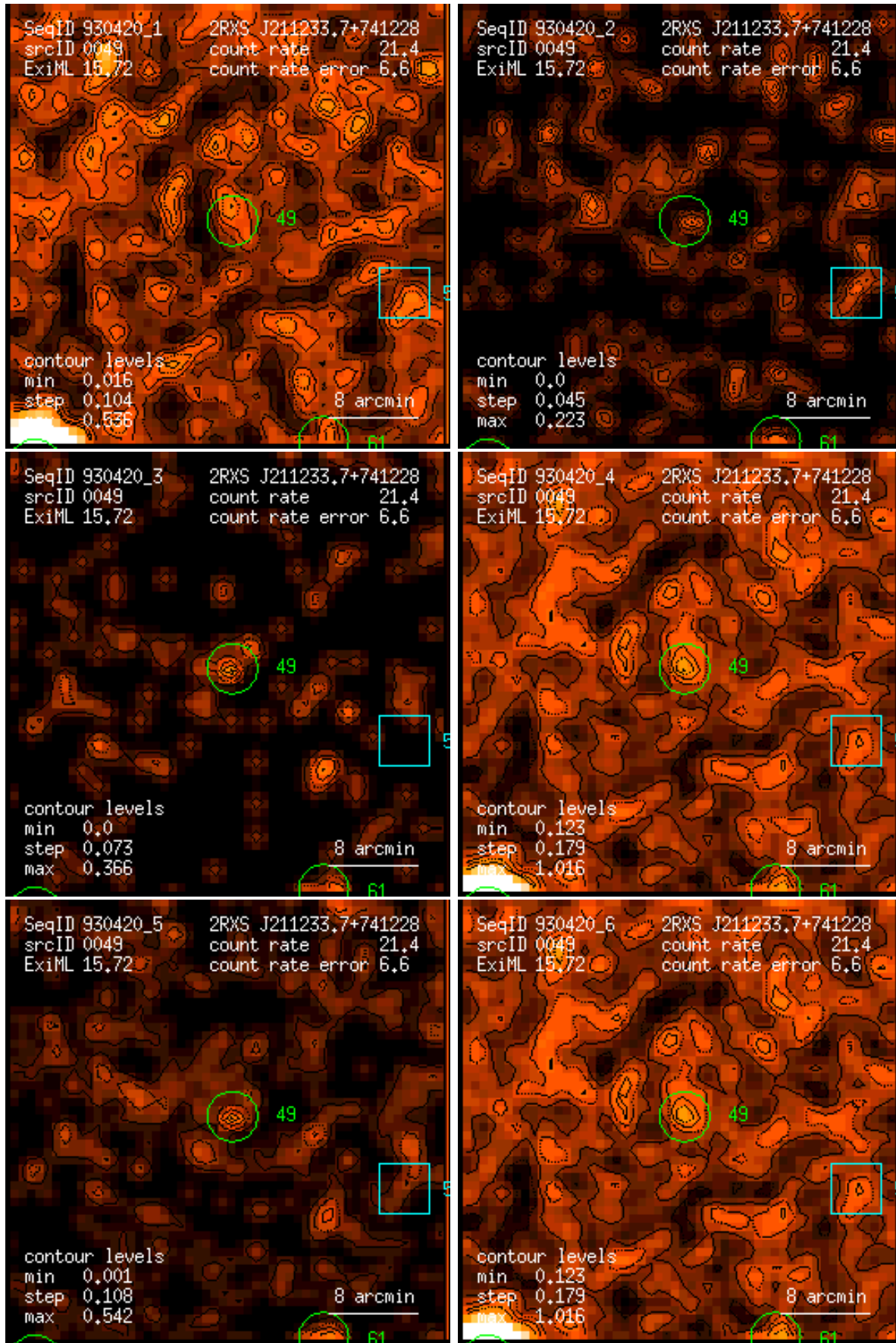
Figure 49: RASS 930420: detection 0049: band rate images, Gaussian filter: (1) PSPC channels 11 – 41, (2) 52 – 90, (3) 91 – 201, (4) 11 – 235, (5) 52 – 201, (6) 11 – 201. Broad band rates in counts/ks. Band rate contour levels in counts/ks/arcmin 2 .
