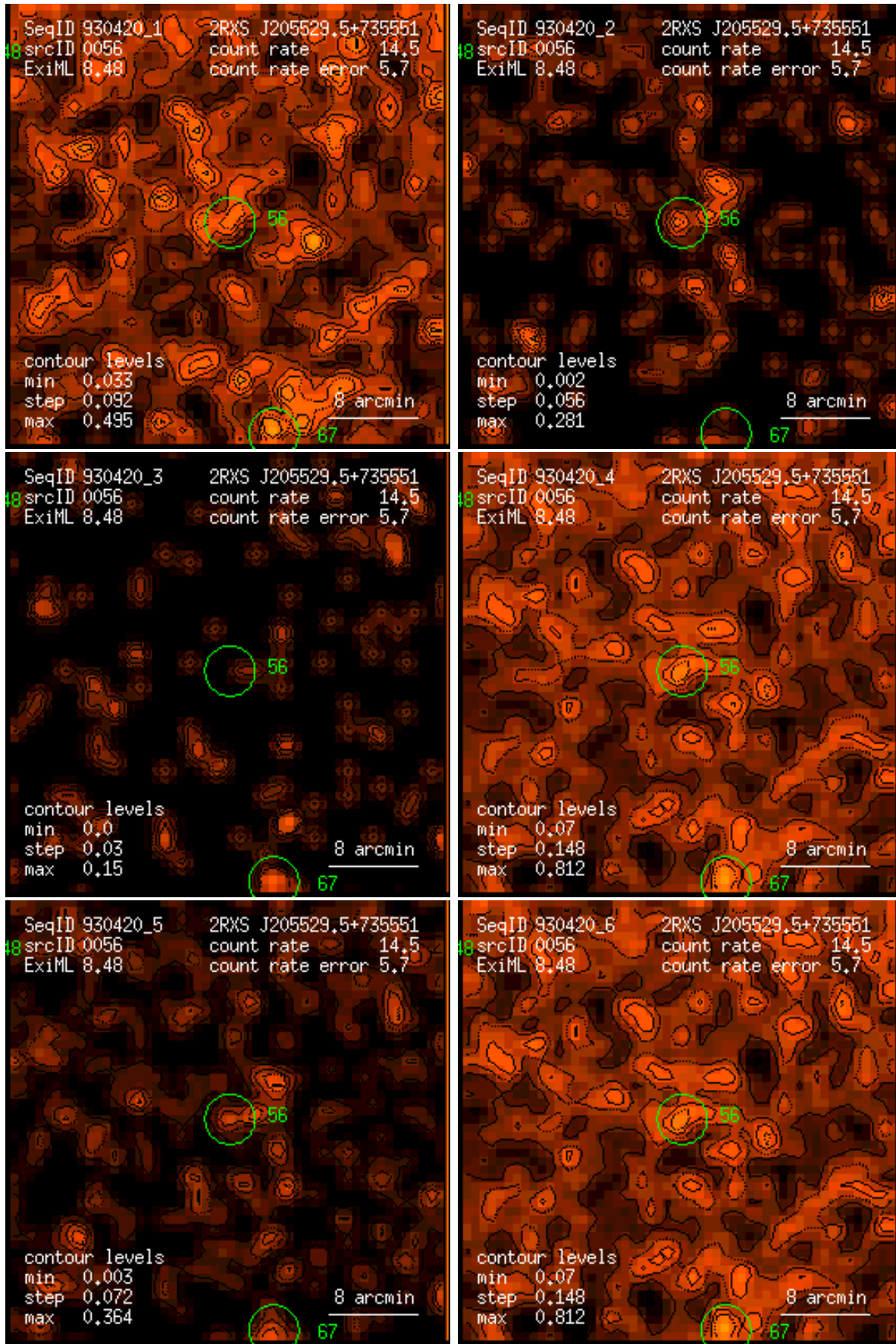
Figure 56: RASS 930420: detection 0056: band rate images, Gaussian filter: (1) PSPC channels 11 – 41, (2) 52 – 90, (3) 91 – 201, (4) 11 – 235, (5) 52 – 201, (6) 11 – 201. Broad band rates in counts/ks. Band rate contour levels in counts/ks/arcmin 2 .
