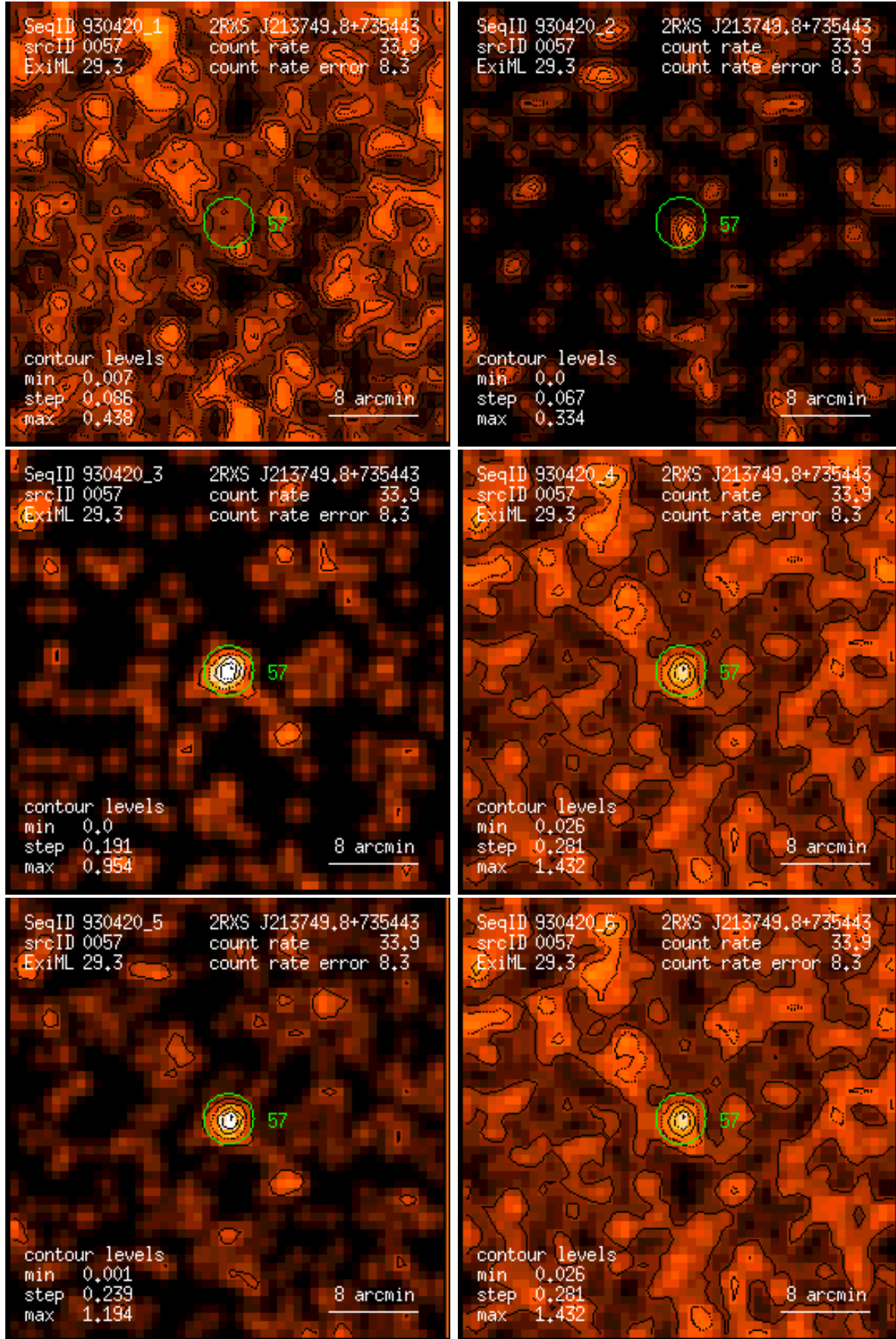
Figure 57: RASS 930420: detection 0057: band rate images, Gaussian filter: (1) PSPC channels 11 – 41, (2) 52 – 90, (3) 91 – 201, (4) 11 – 235, (5) 52 – 201, (6) 11 – 201. Broad band rates in counts/ks. Band rate contour levels in counts/ks/arcmin 2 .
