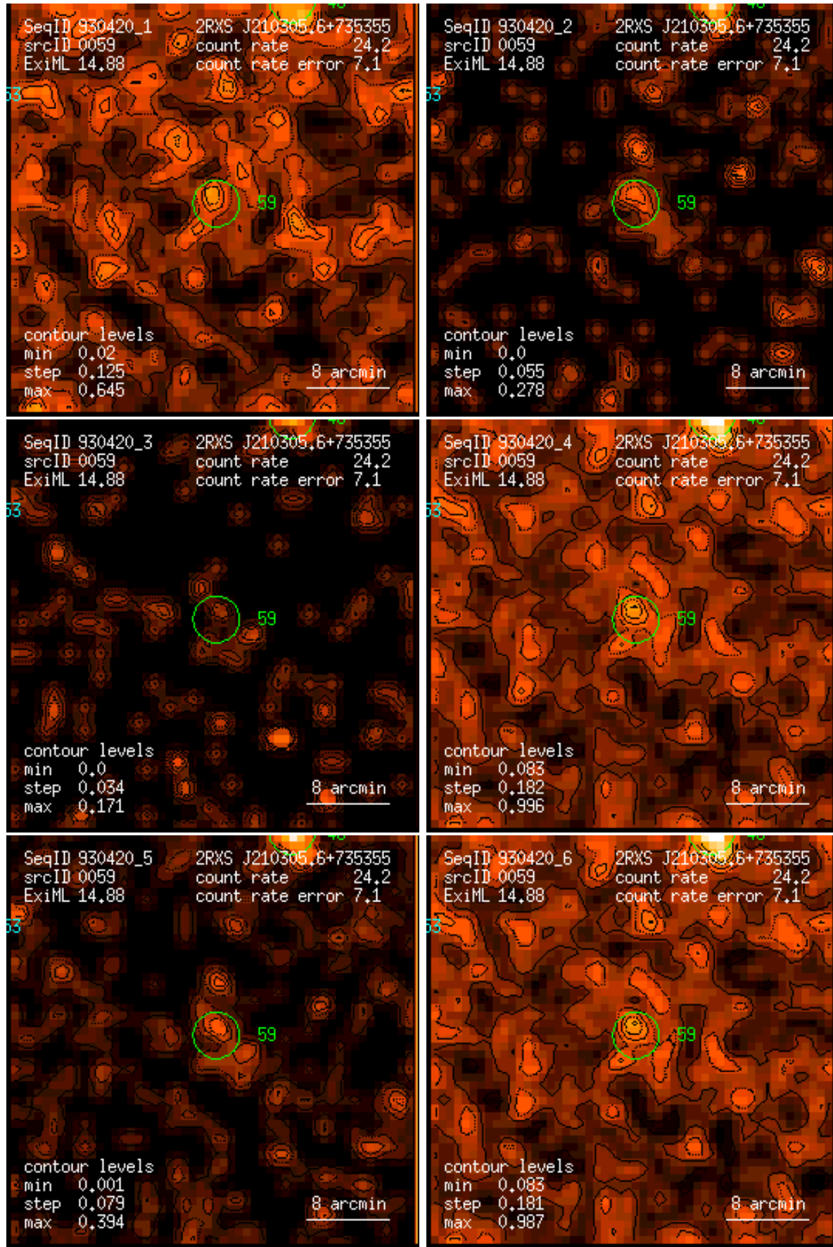
Figure 59: RASS 930420: detection 0059: band rate images, Gaussian filter: (1) PSPC channels 11 – 41, (2) 52 – 90, (3) 91 – 201, (4) 11 – 235, (5) 52 – 201, (6) 11 – 201. Broad band rates in counts/ks. Band rate contour levels in counts/ks/arcmin 2 .
