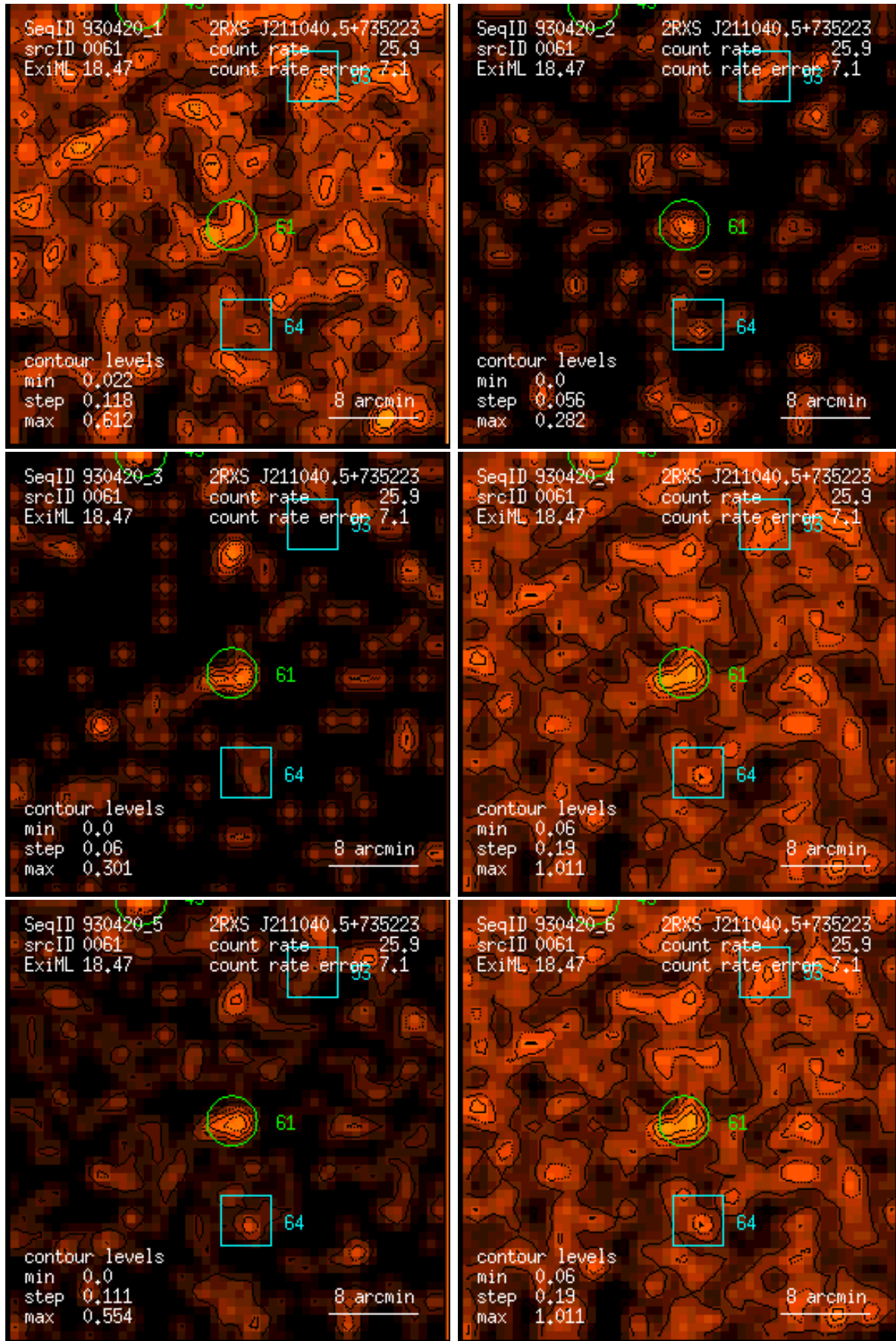
Figure 61: RASS 930420: detection 0061: band rate images, Gaussian filter: (1) PSPC channels 11 – 41, (2) 52 – 90, (3) 91 – 201, (4) 11 – 235, (5) 52 – 201, (6) 11 – 201. Broad band rates in counts/ks. Band rate contour levels in counts/ks/arcmin 2 .
