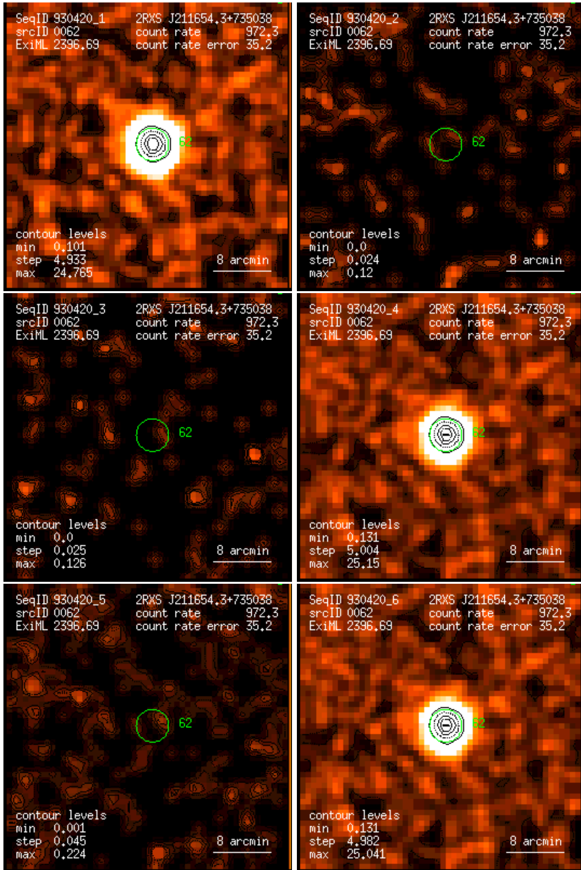
Figure 62: RASS 930420: detection 0062: band rate images, Gaussian filter: (1) PSPC channels 11 – 41, (2) 52 – 90, (3) 91 – 201, (4) 11 – 235, (5) 52 – 201, (6) 11 – 201. Broad band rates in counts/ks. Band rate contour levels in counts/ks/arcmin 2 .
