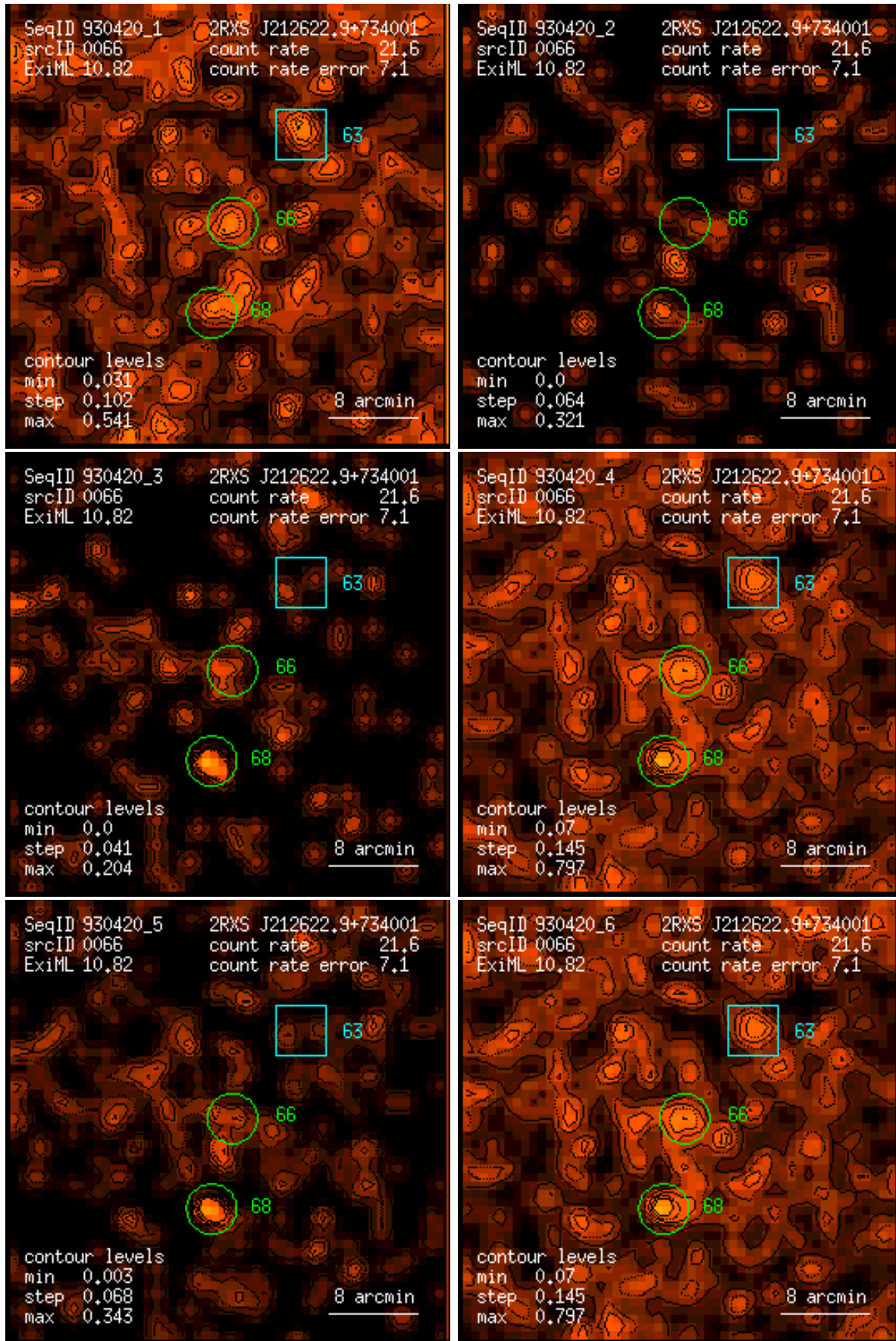
Figure 66: RASS 930420: detection 0066: band rate images, Gaussian filter: (1) PSPC channels 11 – 41, (2) 52 – 90, (3) 91 – 201, (4) 11 – 235, (5) 52 – 201, (6) 11 – 201. Broad band rates in counts/ks. Band rate contour levels in counts/ks/arcmin 2 .
