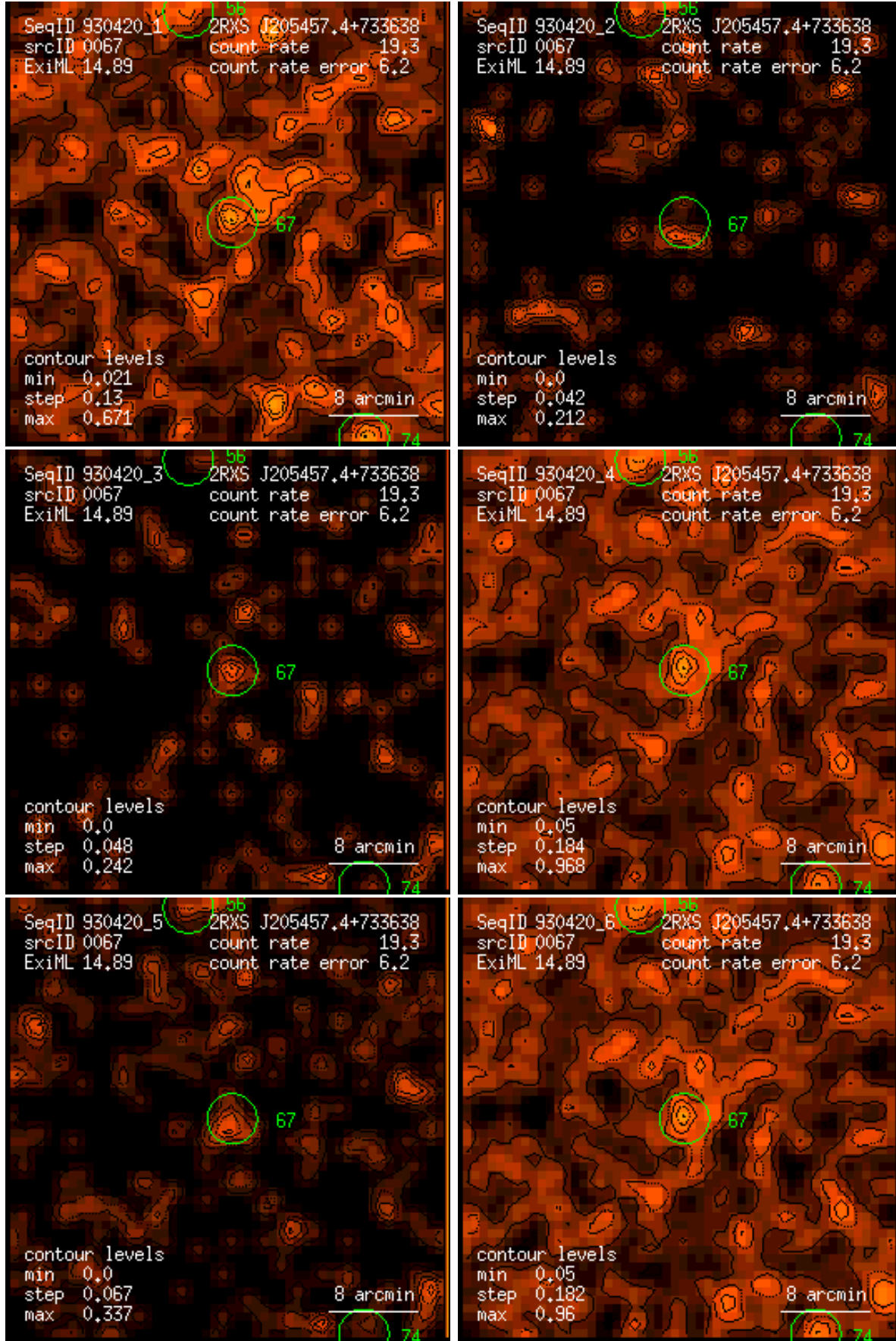
Figure 67: RASS 930420: detection 0067: band rate images, Gaussian filter: (1) PSPC channels 11 – 41, (2) 52 – 90, (3) 91 – 201, (4) 11 – 235, (5) 52 – 201, (6) 11 – 201. Broad band rates in counts/ks. Band rate contour levels in counts/ks/arcmin 2 .
