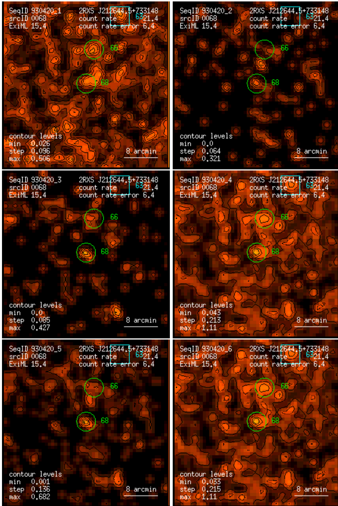
Figure 68: RASS 930420: detection 0068: band rate images, Gaussian filter: (1) PSPC channels 11 – 41, (2) 52 – 90, (3) 91 – 201, (4) 11 – 235, (5) 52 – 201, (6) 11 – 201. Broad band rates in counts/ks. Band rate contour levels in counts/ks/arcmin 2 .
