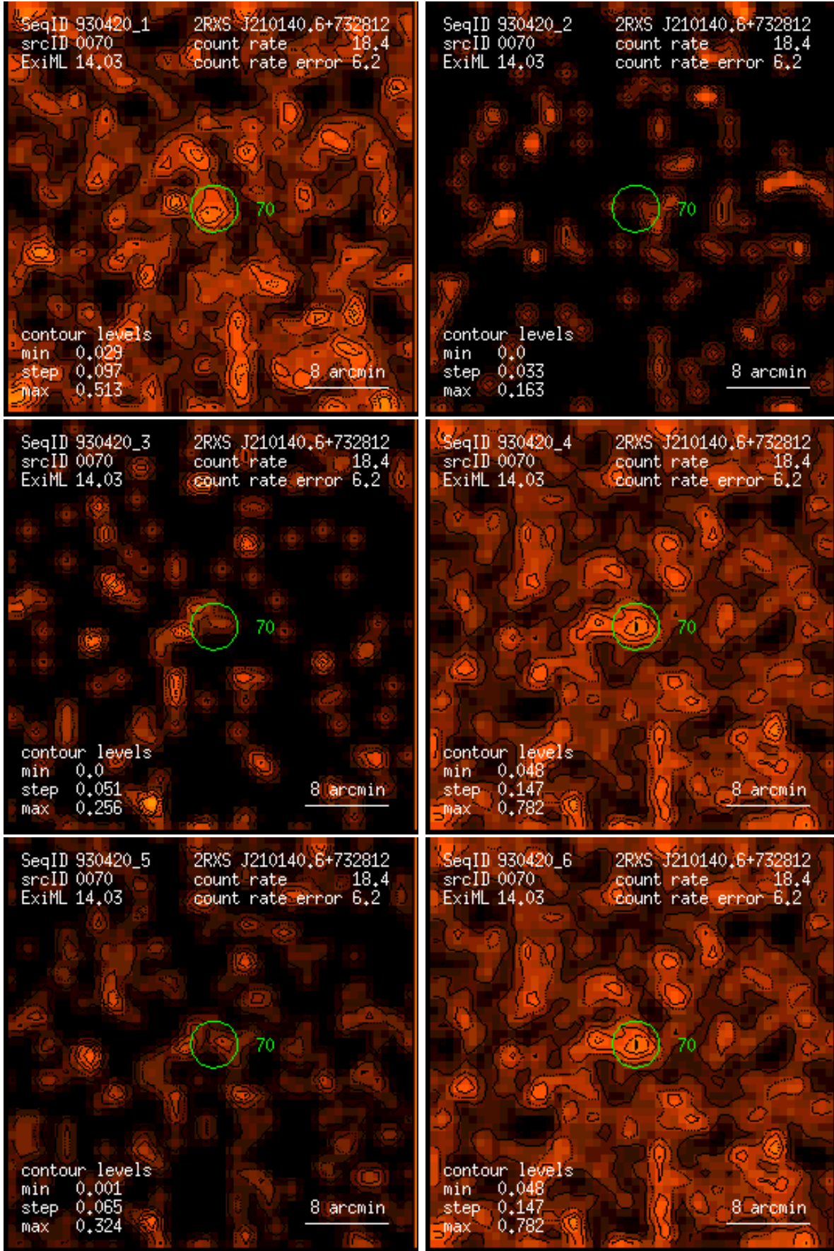
Figure 70: RASS 930420: detection 0070: band rate images, Gaussian filter: (1) PSPC channels 11 – 41, (2) 52 – 90, (3) 91 – 201, (4) 11 – 235, (5) 52 – 201, (6) 11 – 201. Broad band rates in counts/ks. Band rate contour levels in counts/ks/arcmin 2 .
