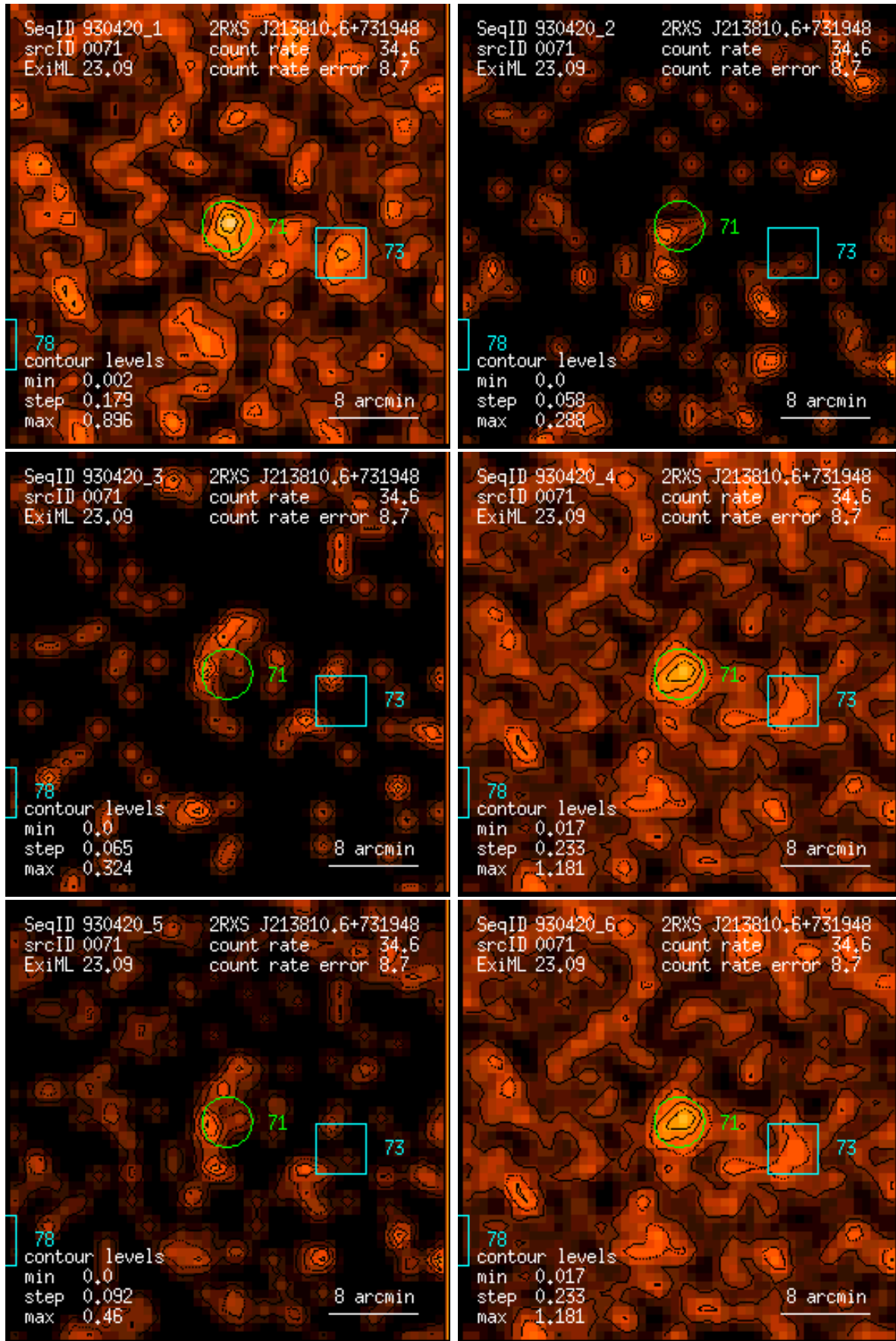
Figure 71: RASS 930420: detection 0071: band rate images, Gaussian filter: (1) PSPC channels 11 – 41, (2) 52 – 90, (3) 91 – 201, (4) 11 – 235, (5) 52 – 201, (6) 11 – 201. Broad band rates in counts/ks. Band rate contour levels in counts/ks/arcmin 2 .
