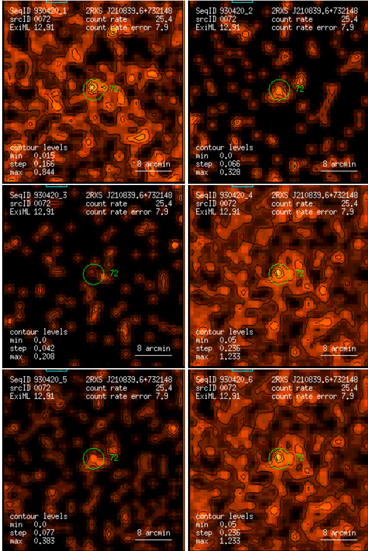
Figure 72: RASS 930420: detection 0072: band rate images, Gaussian filter: (1) PSPC channels 11 – 41, (2) 52 – 90, (3) 91 – 201, (4) 11 – 235, (5) 52 – 201, (6) 11 – 201. Broad band rates in counts/ks. Band rate contour levels in counts/ks/arcmin 2 .
