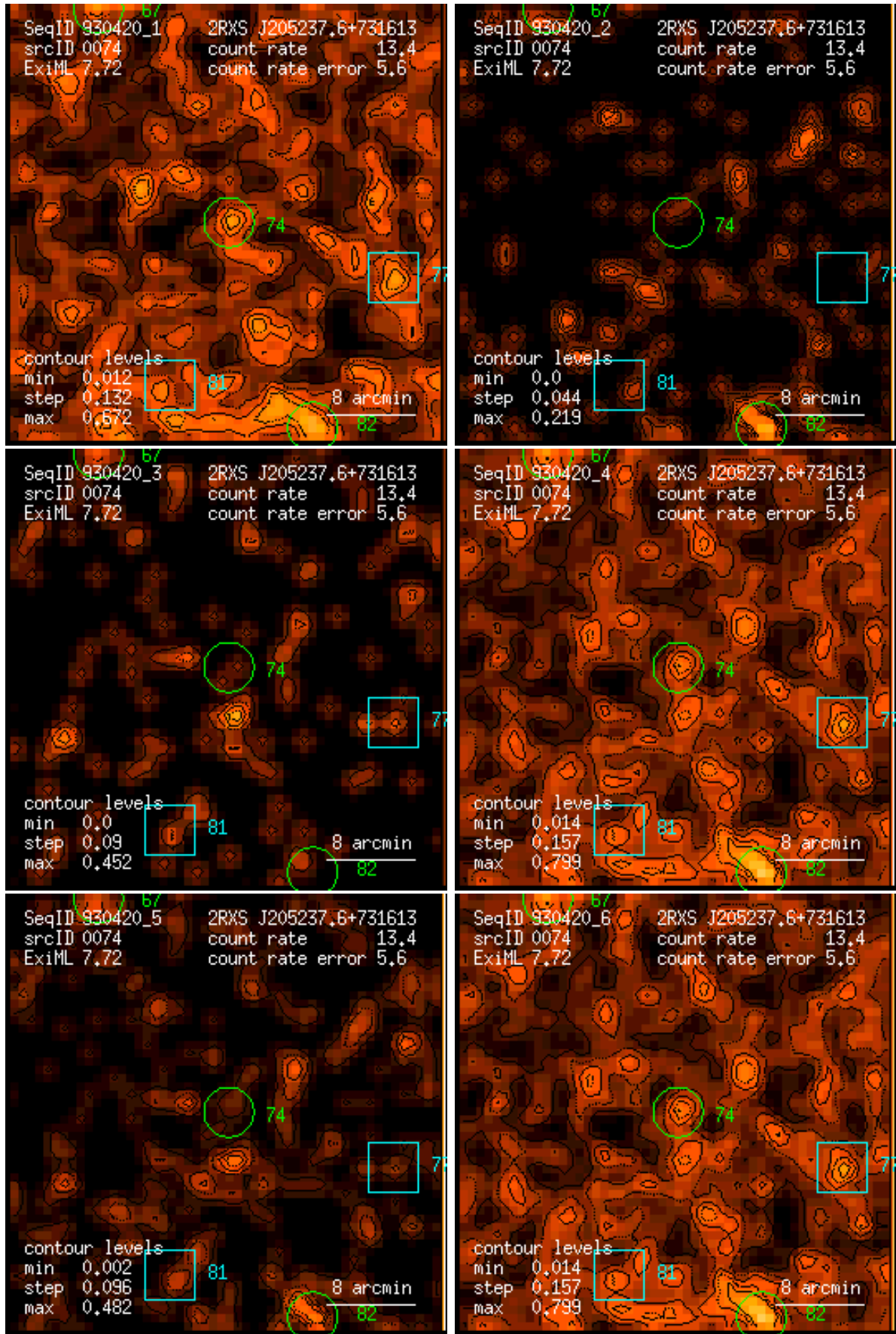
Figure 74: RASS 930420: detection 0074: band rate images, Gaussian filter: (1) PSPC channels 11 – 41, (2) 52 – 90, (3) 91 – 201, (4) 11 – 235, (5) 52 – 201, (6) 11 – 201. Broad band rates in counts/ks. Band rate contour levels in counts/ks/arcmin 2 .
