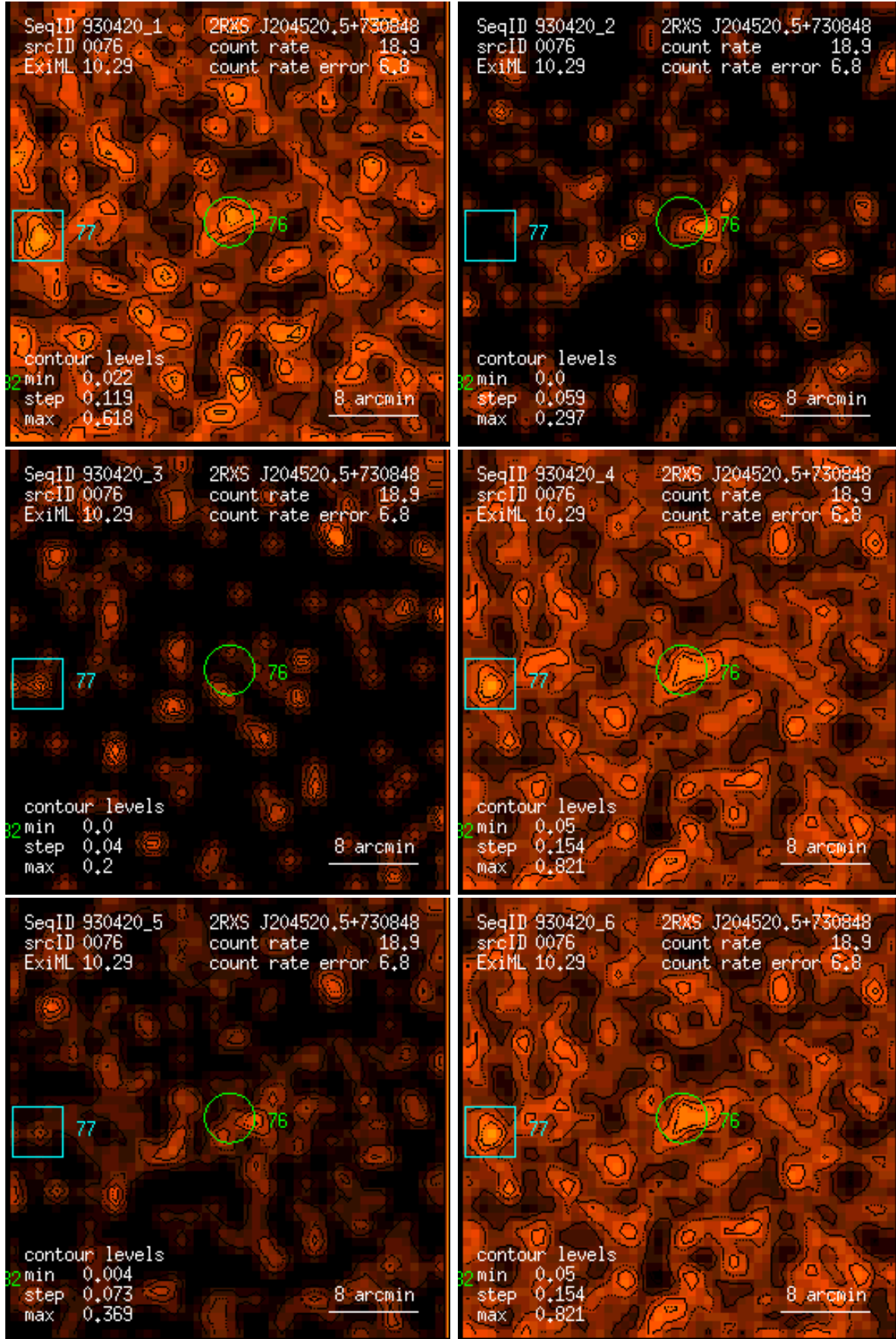
Figure 76: RASS 930420: detection 0076: band rate images, Gaussian filter: (1) PSPC channels 11 – 41, (2) 52 – 90, (3) 91 – 201, (4) 11 – 235, (5) 52 – 201, (6) 11 – 201. Broad band rates in counts/ks. Band rate contour levels in counts/ks/arcmin 2 .
